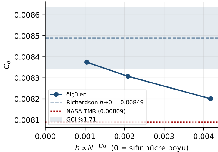
NACA0012 \alpha = 0^\circ — 2B C-grid p = 0.666 , asimptotik oran 0.992
