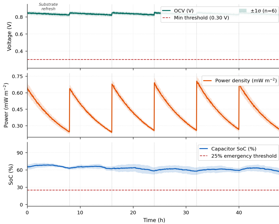
Figure 2. Physics-based 48-hour simulation results (Scenario A parameters, Table 1): (top) open-circuit voltage derived from the Nernst equation with natural substrate replenishment via rhizosphere organic influx; (middle) resulting power density; (bottom) supercapacitor state of charge with duty-cycle discharge events. SoC remaining above 30% demonstrates that the 10-minute cycle is viable.
