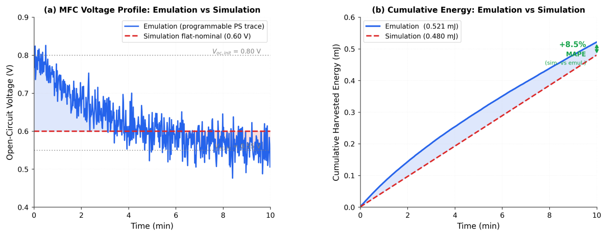
Figure 10. Power-trace emulation validation. (a) MFC open-circuit voltage profile over one 10-minute duty cycle: emulation trace (blue, V_{oc\_init} = 0.80 V decaying with \tau = 180 s) vs. flat-nominal simulation model (red dashed, 0.60 V). Shaded regions indicate deviation from the nominal assumption. (b) Cumulative harvested energy: the trace-based emulation yields 0.521 mJ vs. 0.480 mJ for the flat-nominal model (MAPE = +8.5%), confirming the simulation is a conservative lower bound.
