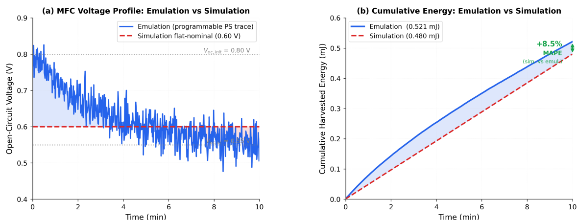
Figure 9. Power-trace emulation validation. (a) MFC open-circuit voltage profile over one 10-minute duty cycle: emulation trace (blue, V_{oc\_init} = 0.80 V decaying with \tau = 180 s) vs. flat-nominal simulation model (red dashed, 0.60 V). Shaded regions indicate deviation from the nominal assumption. (b) Cumulative harvested energy: the trace-based emulation yields 0.521 mJ vs. 0.480 mJ for the flat-nominal model (MAPE = +8.5%), confirming the simulation is a conservative lower bound.
