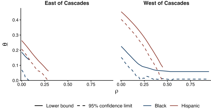
Figure 9: Sensitivity to violations of Assumption 2, by side of the Cascade crest. Solid lines are \hat{\theta}_{0,\rho} and dashed lines the one-sided 95% confidence limit. Curves terminate where the confidence limit reaches zero.
