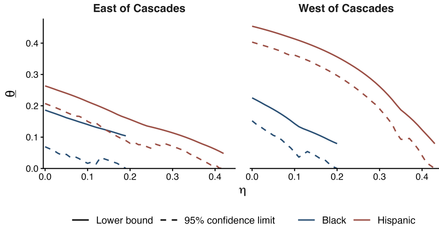
Figure 8: Sensitivity to violations of Assumption 1, by side of the Cascade crest. Solid lines are \hat{\theta}_{\eta,0} and dashed lines the one-sided 95% confidence limit. Curves are truncated where the confidence limit reaches zero.
