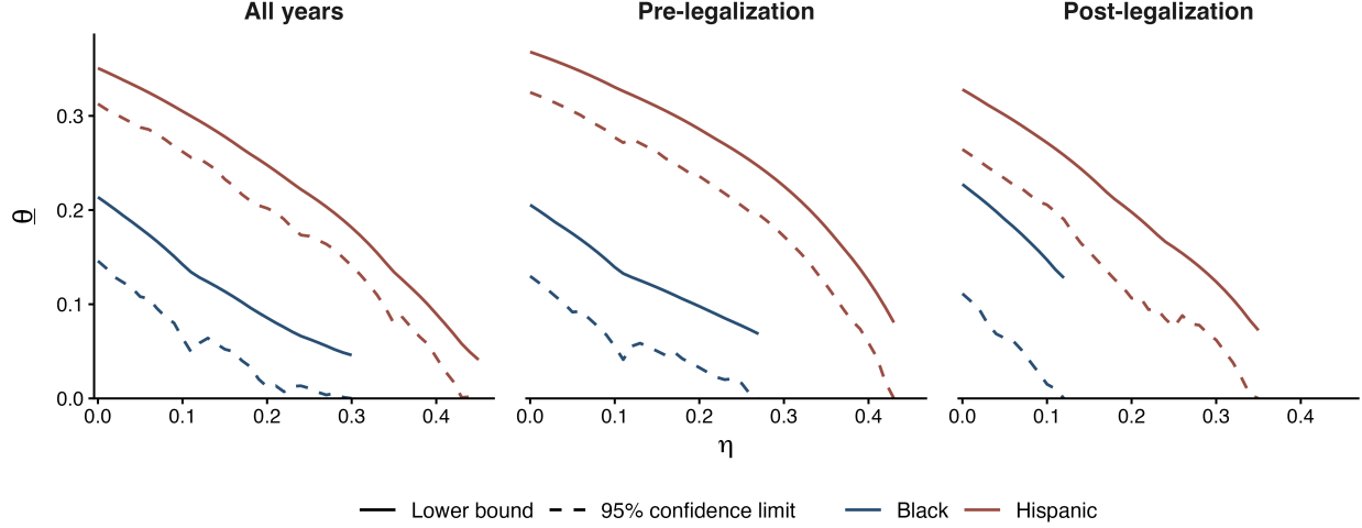
Figure 6: Sensitivity of the lower bound to violations of Assumption 1. Solid lines give \hat{\theta}_{\eta,0} and dashed lines the one-sided 95% confidence limit, as \eta varies with \rho held at zero. Curves terminate where the confidence limit reaches zero, beyond which the data are uninformative about the sign of the bound.
