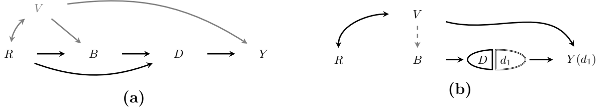
Figure 3: A Single World Intervention Graph describing the data-generating process in equilibrium. Panel (a) depicts the full causal model for convenience of comparison. Panel (b) gives a Single World Intervention Graph describing the data-generating process in equilibrium. The hypothesis of no taste-based discrimination is reflected by the absence of an edge R \rightarrow D . The model implies that all searched individuals are marginal, which additionally removes the edge V \rightarrow B , removing all heterogeneity in beliefs.
