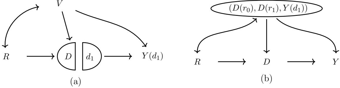
Figure 5: A new motivation for the outcome test. Panel (a): intervening on search, a SWIG is drawn for the data-generating process (suppressing officer beliefs), revealing graphically that Y(d_1) is a negative control outcome for D . Panel (b) shows how we may without loss represent V by the relevant principal strata; recall that Y(d_0) = 0 in this setting.
