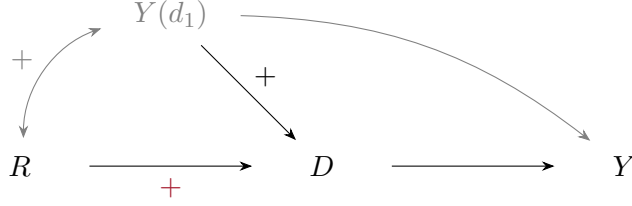
Figure 2: Conditioning on a collider. Under officer clairvoyance, B = Y(d_1) , it suffices to take the confounder V = Y(d_1) . The goal of the test is to detect if R has a positive effect on D , indicated by the red + . Hit rates condition on the collider D , forcing the analyst to wrestle with several interaction effects to infer discrimination. Conditions (i) and (ii) of Proposition 3 is reflected graphically by the ‘ + ’ signs on the relevant edges using notation from the signed graphs literature (VanderWeele and Robins, 2010).
