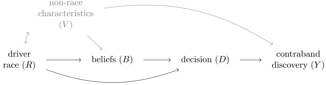
Figure 1: Causal graph for contraband search. Non-race characteristics about the encounter inform an officer’s beliefs about the likelihood of discovering contraband, possibly leading to a search. Disparities in the effect of R on D decompose into taste-based discrimination ( R \rightarrow D ) and statistical discrimination ( R \rightarrow B \rightarrow D ). exogenous disturbances are suppressed.
