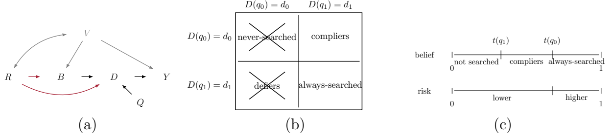
Figure 4: Illustration of Anwar and Fang test. (a) The DGP. (b) Principal strata on D in the absence of discrimination. (c) Mapping from beliefs to strata, with corresponding risk, if beliefs are calibrated. Under the null, the red arrows (those emanating from R ) in (a) vanish, and suppose for hypothesis that D(q) is monotonic in q , so that among those searched, we have no never-takers or defiers. Equally, the White ( q_0 ) officer's threshold is higher than the minority ( q_1 ) officer's threshold, see (c). Assuming beliefs are calibrated, the contraband risk among minority officer searches is lower than that of White officers.
