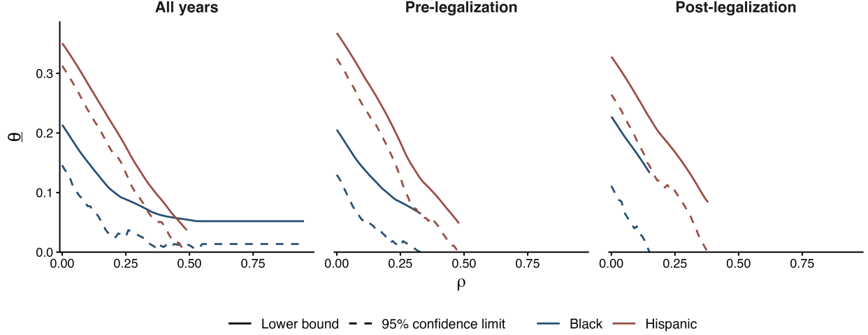
Figure 7: Sensitivity of the lower bound to violations of Assumption 2. Solid lines give \hat{\theta}_{0,\rho} and dashed lines the one-sided 95% confidence limit, as \rho varies with \eta held at zero. Curves terminate where the confidence limit reaches zero. The Black curve plateaus because \rho scales only the first branch of (17) and cannot erode contexts in which Black searches are the more productive.
