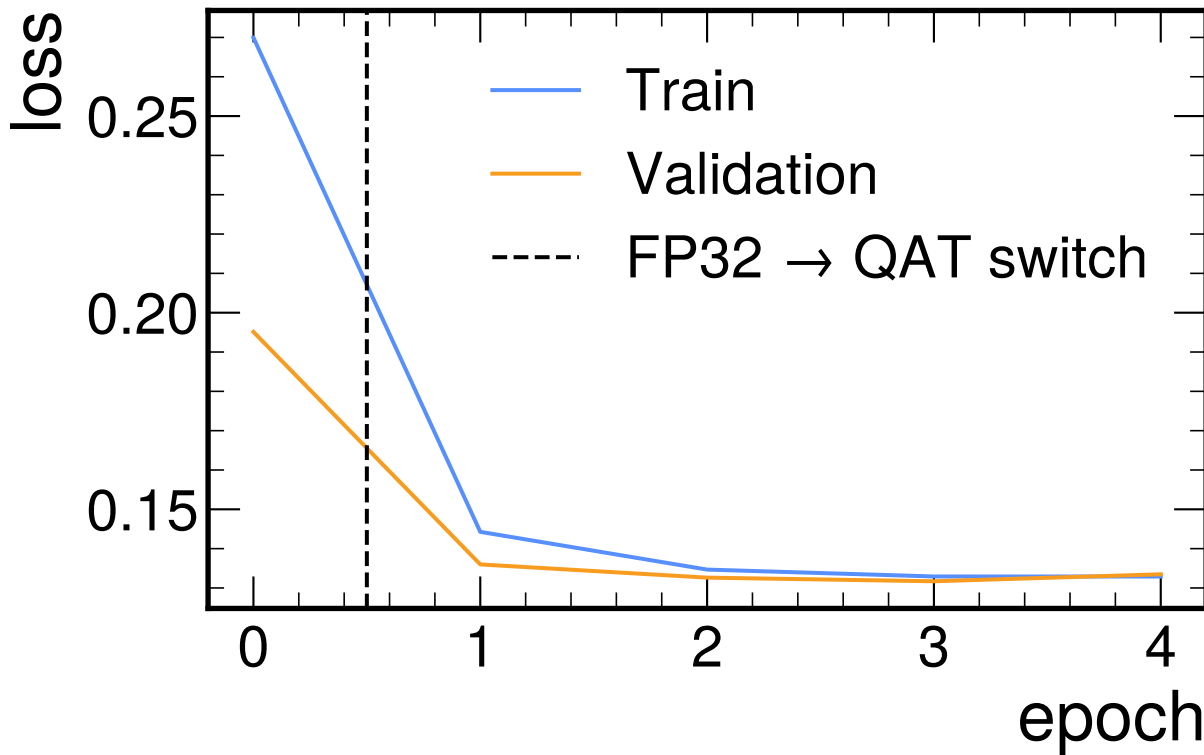
BitNet Model Loss
