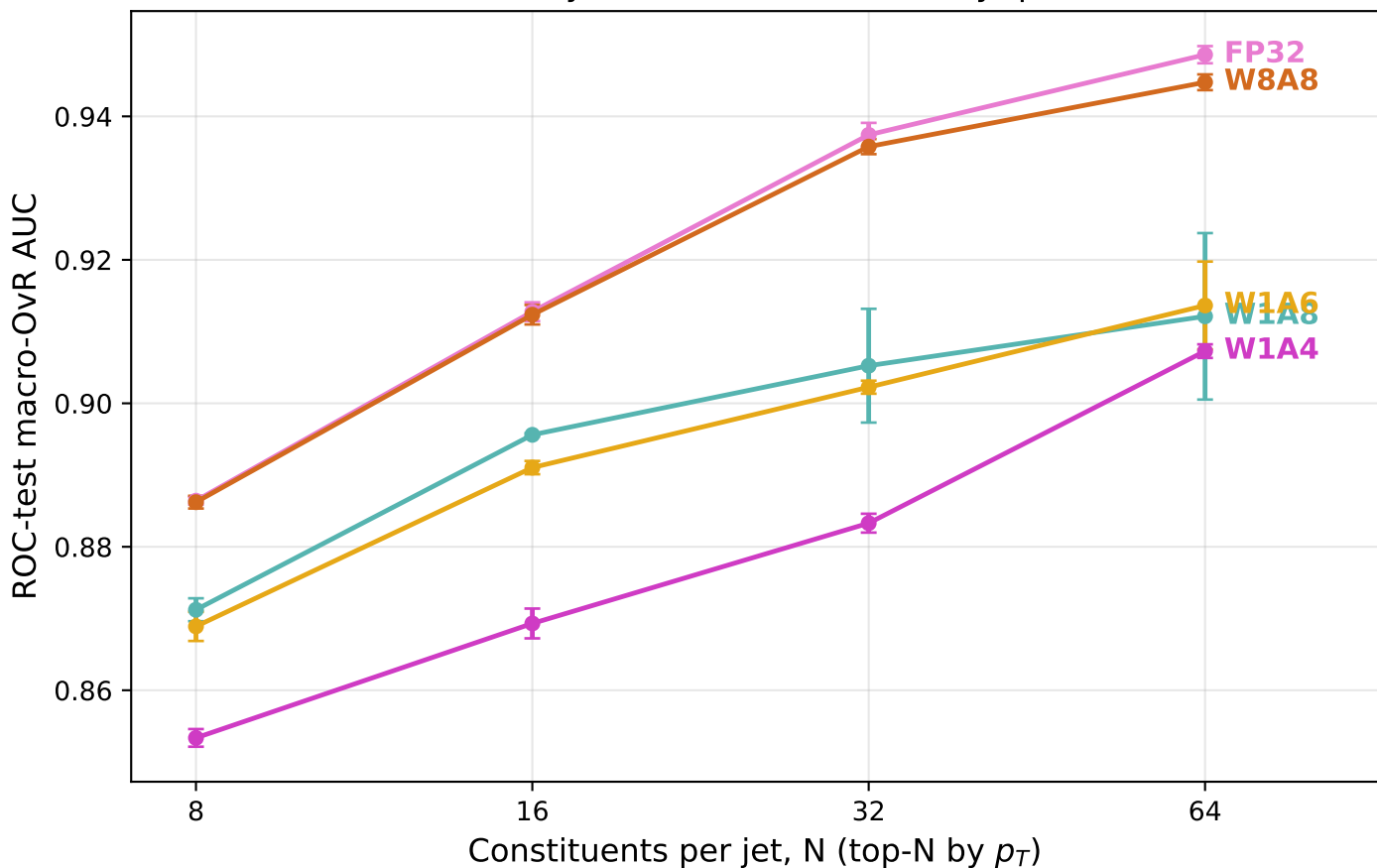
Round 14 — accuracy vs constituent count, by quantization arm
