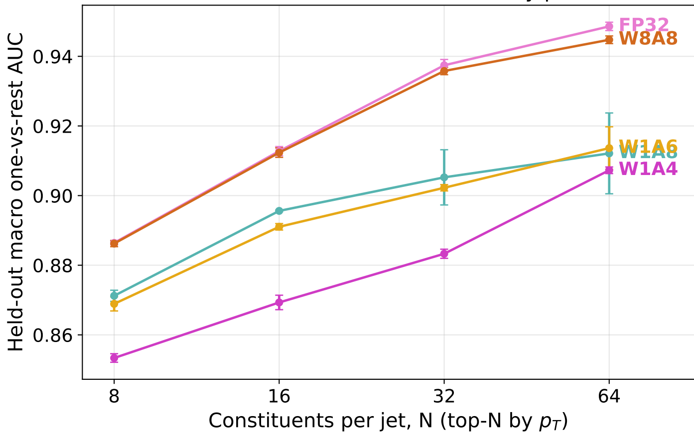
Held-out AUC vs constituent count, by precision
