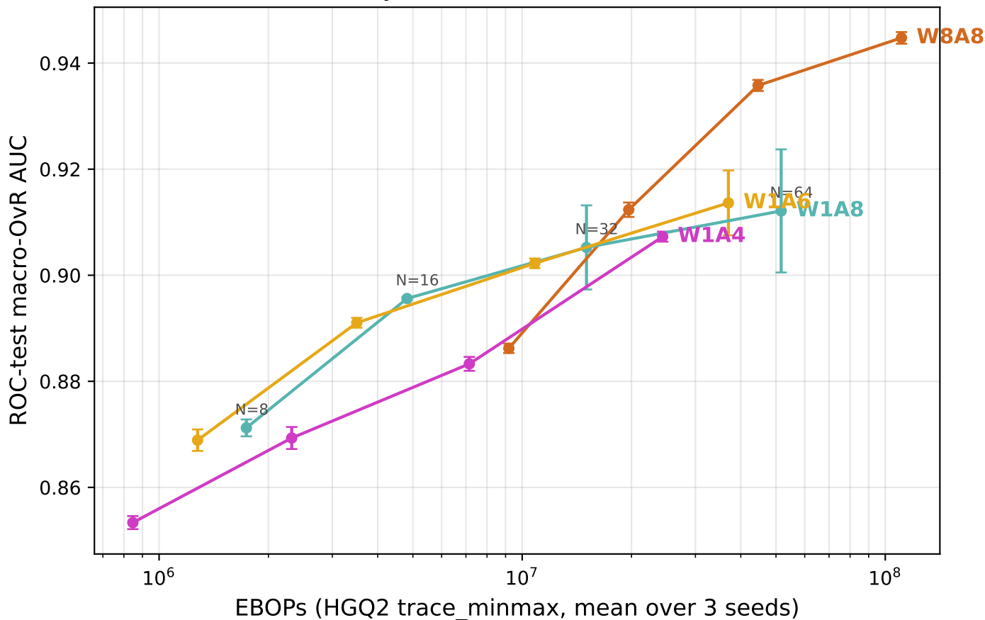
Round 14 — accuracy vs estimated hardware cost (Pareto view)
