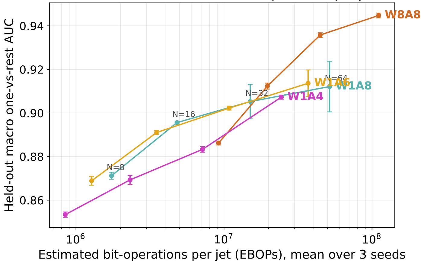
Held-out AUC vs estimated bit-operations per jet
