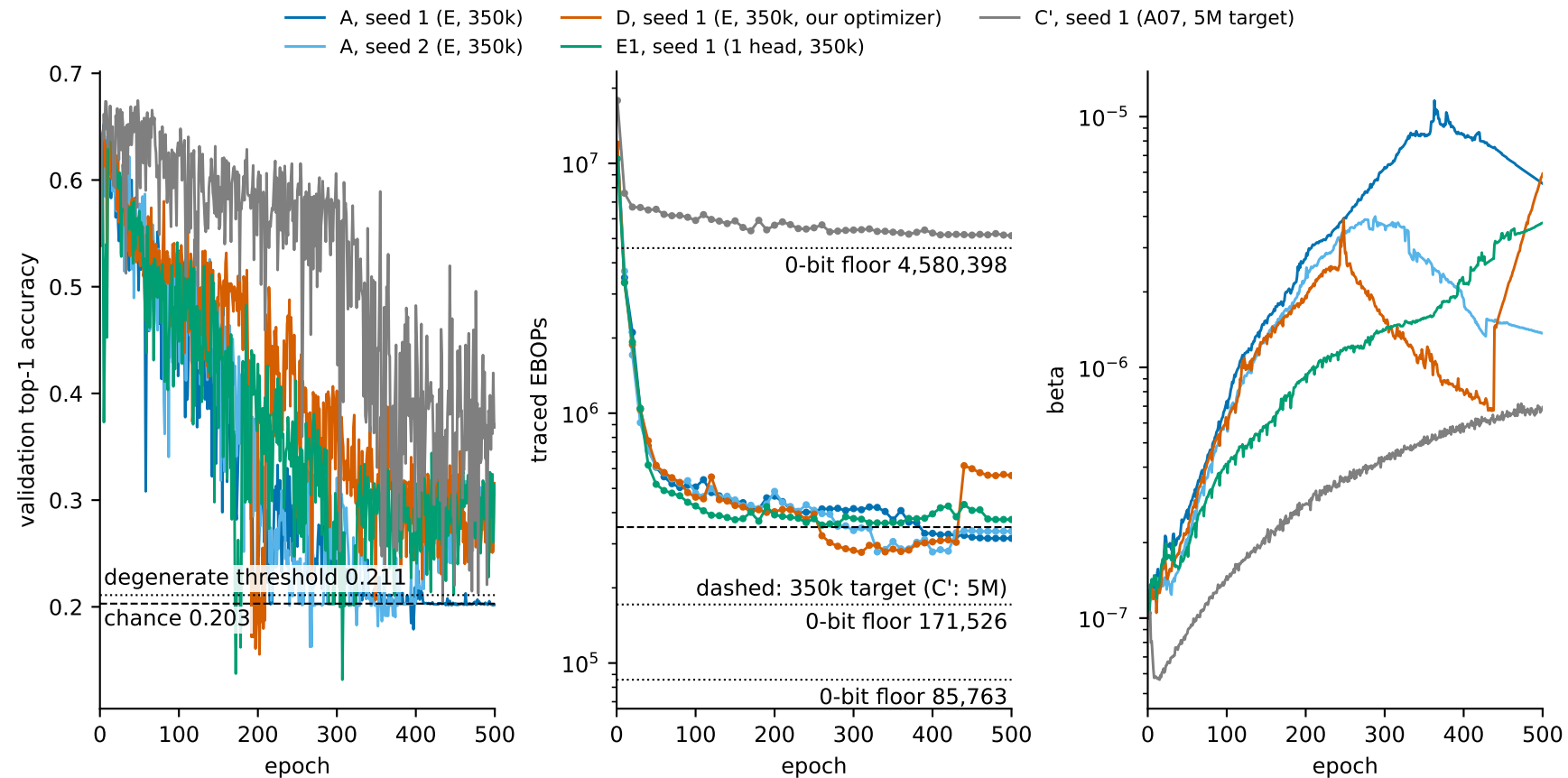
Validation split, n = 62,000 ; pilot b5, single seed per arm (A: two), values read from training logs, not verified.
