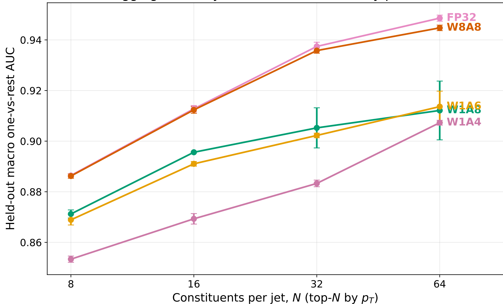
Tagging accuracy vs constituent count, by precision
