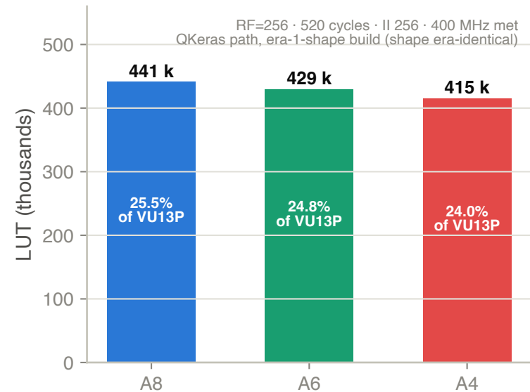
Binary FFN block — DSP = 0 at all precisions
