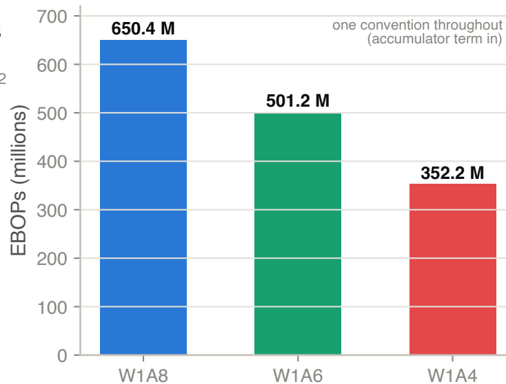
Compute — EBOPs (HGQ2-native)
