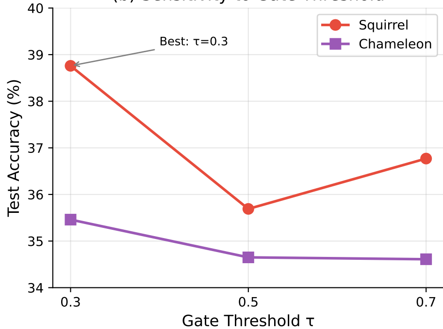
(b) Sensitivity to Gate Threshold
