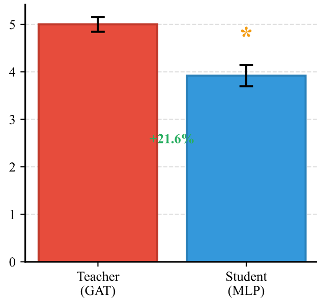
Compactness Ratio (↓ Lower is Better)
