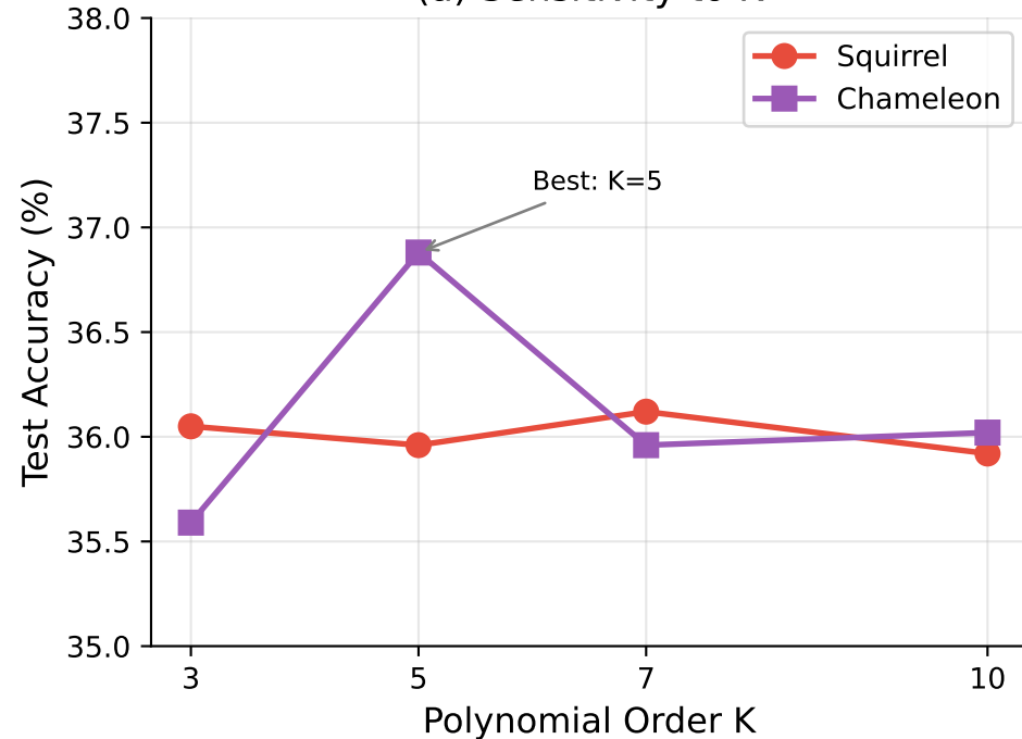
(a) Sensitivity to K
