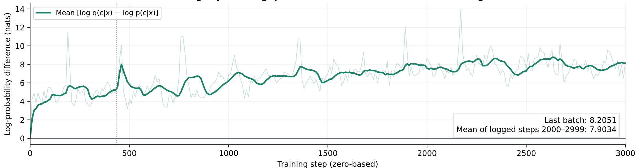
A larger positive gap does not establish better conditioning
