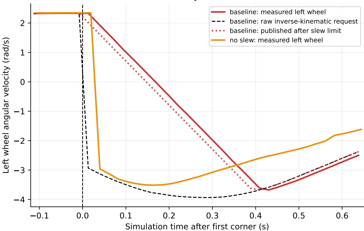
C. A limiter delays wheel reversal
