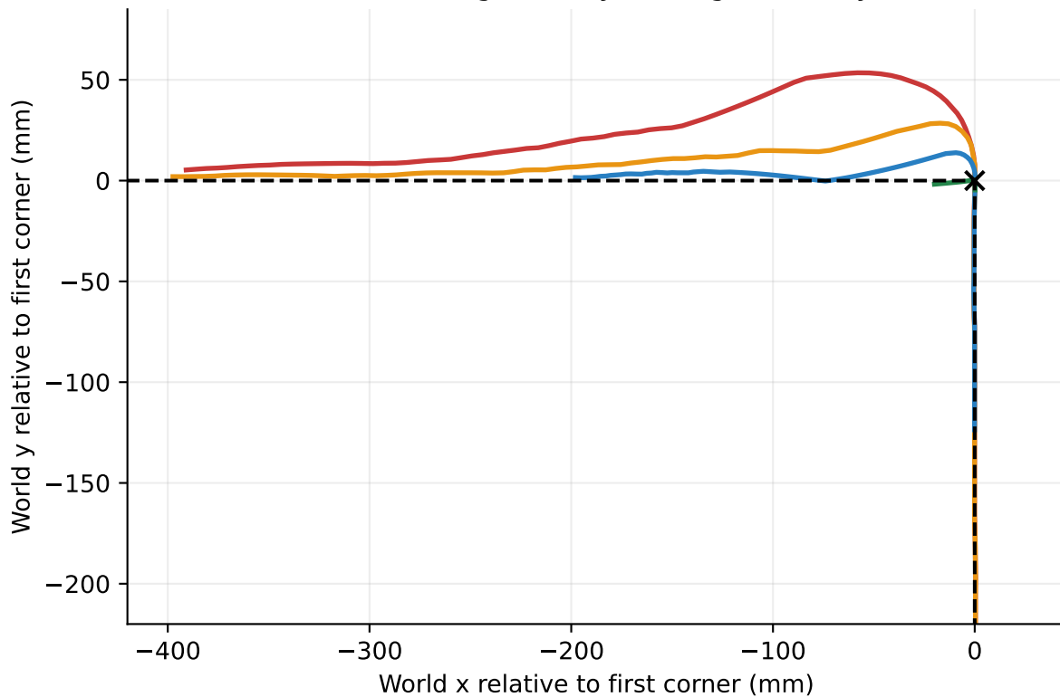
C. A limiter delays wheel reversal
