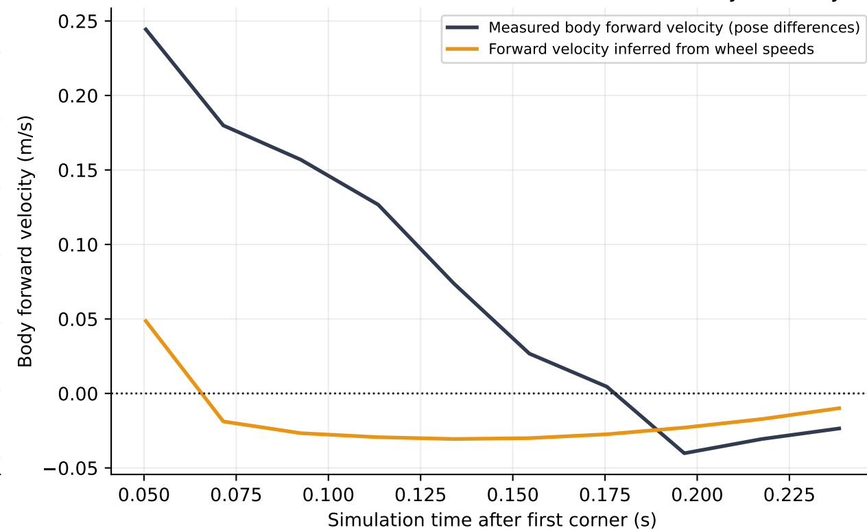
D. No slew limit: wheel reversal does not reverse body instantly
