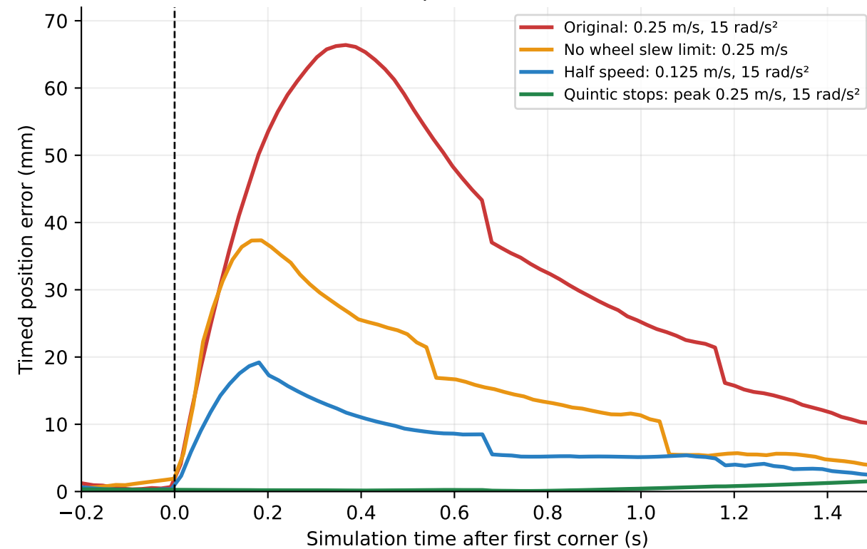
D. No slew limit: wheel reversal does not reverse body instantly
