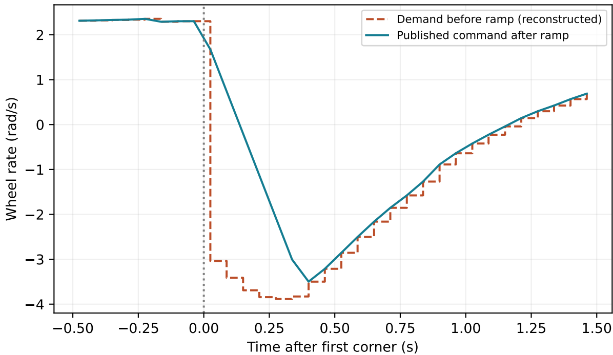
Left wheel: 15 rad/s 2 command ramp
