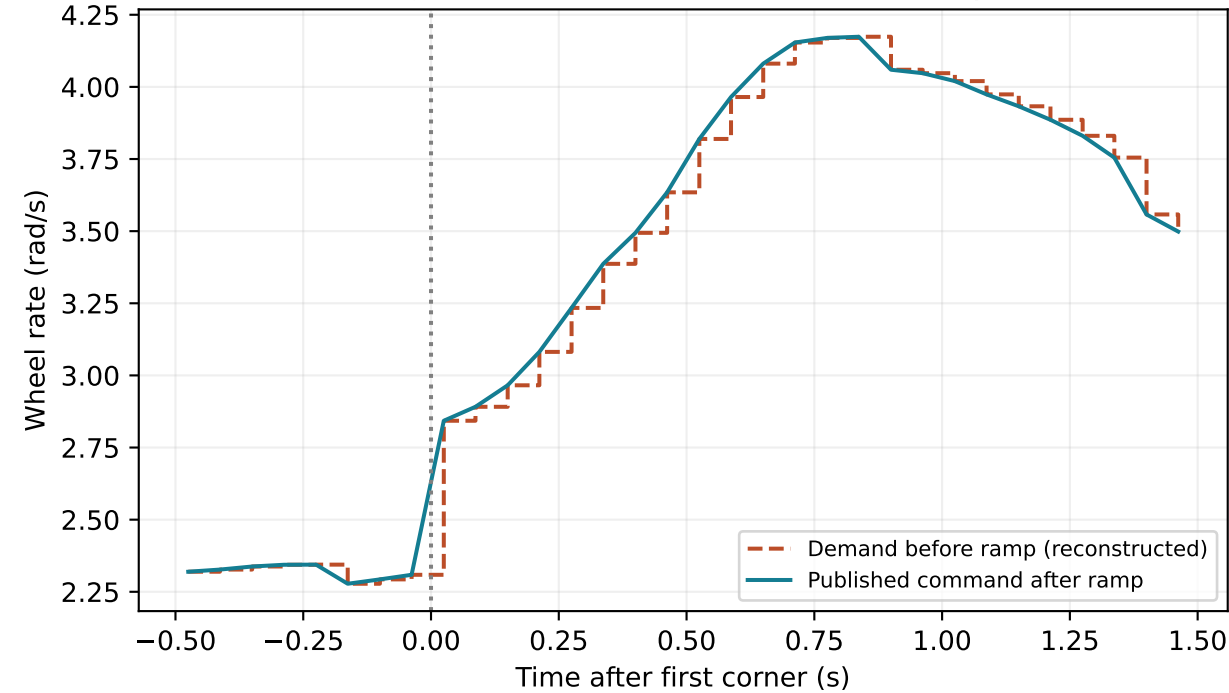
Right wheel: 15 rad/s 2 command ramp
