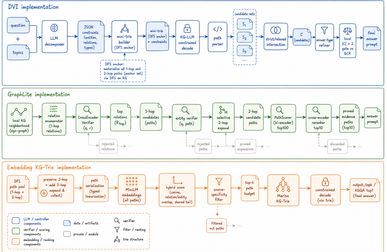
Figure 2: Implementation-level method architecture. Unlike the project overview, this figure expands each method into internal modules, intermediate data structures, and control decisions: DVI tracks constraints and candidate sets, GraphLite replaces KG-LLM decoding with relation/entity/path verifiers, and embedding-guided KG-Trie ranks and budgets paths before trie construction.
