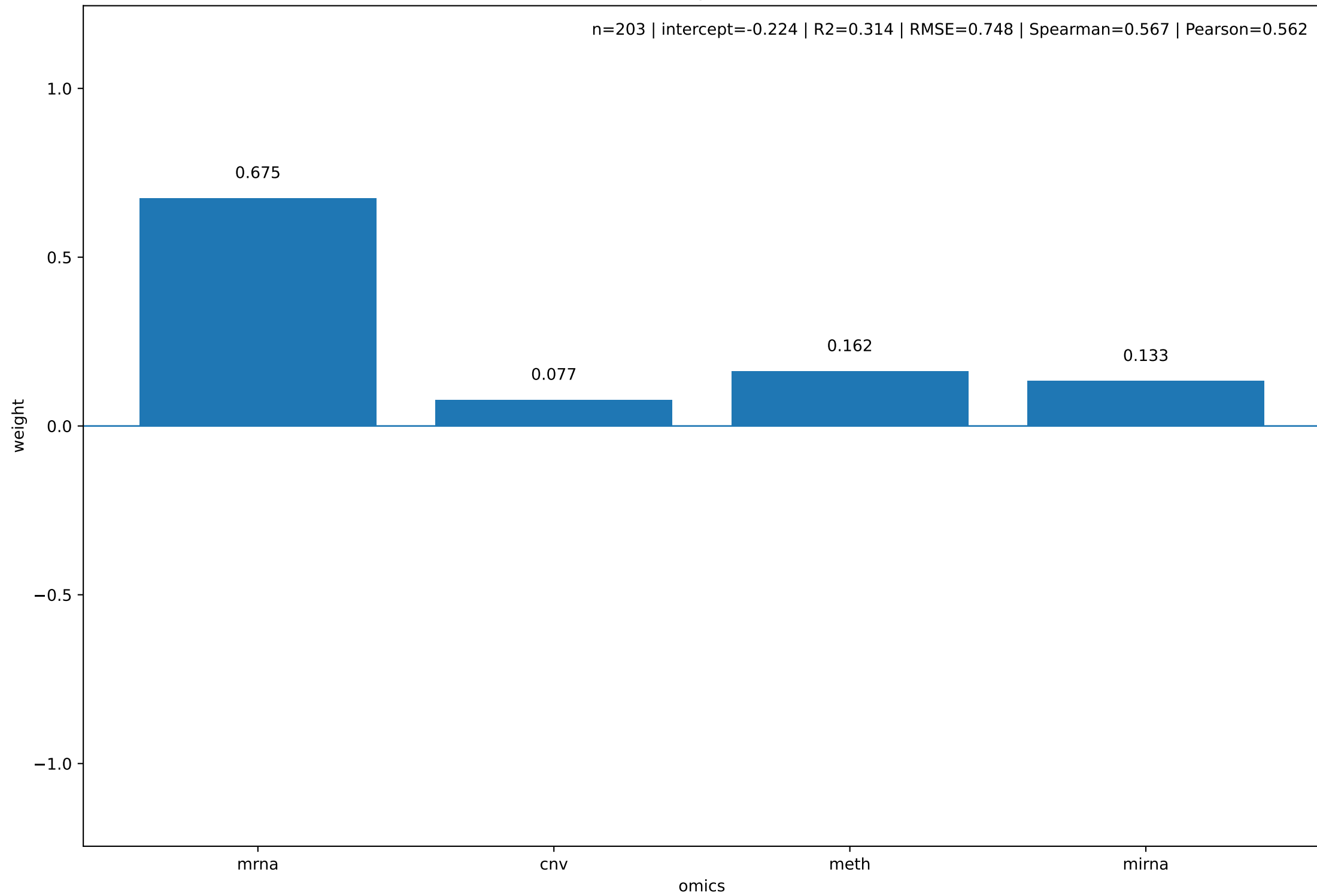
Final omics weights - SB216763
