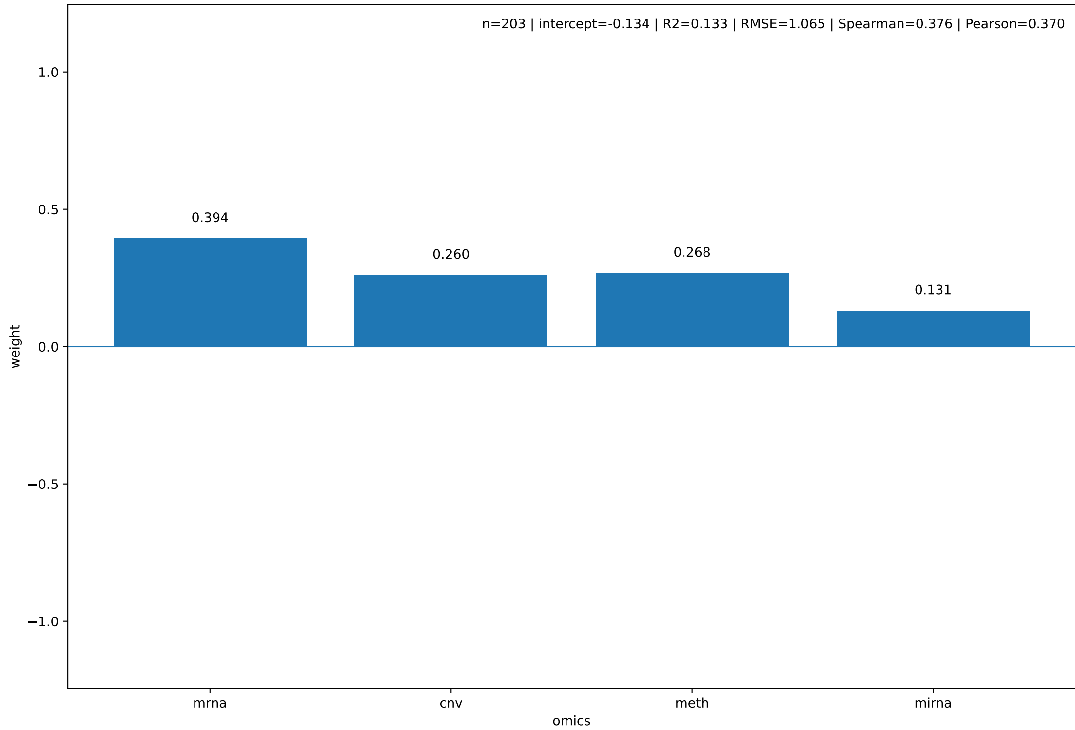
Final omics weights - PFI-1
