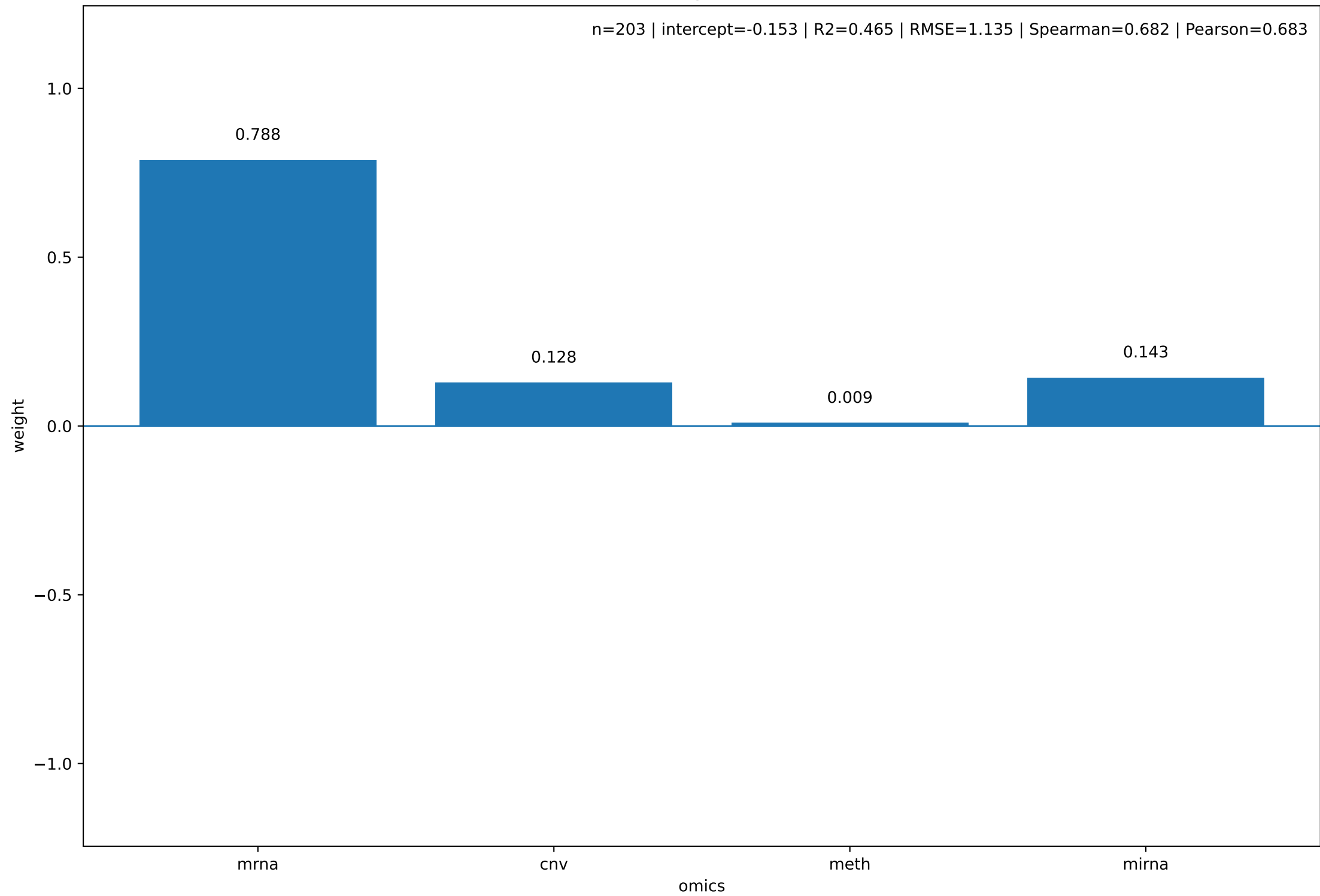
Final omics weights - BOSUTINIB
