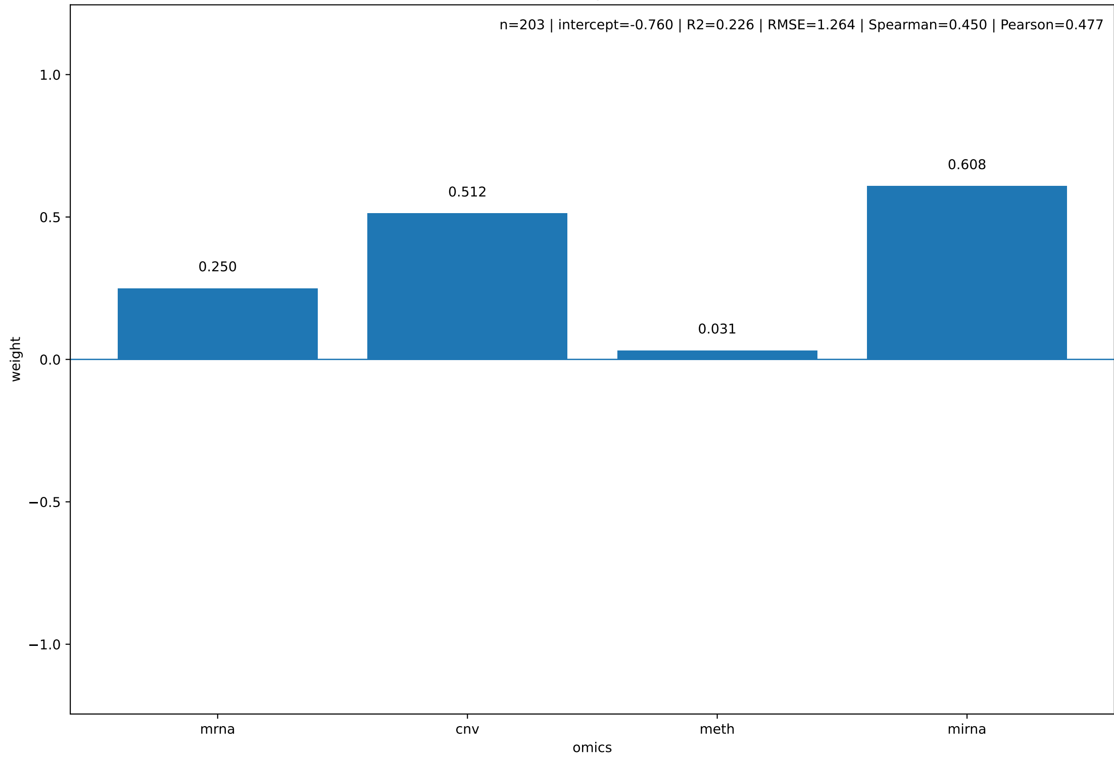
Final omics weights - MK-2206
