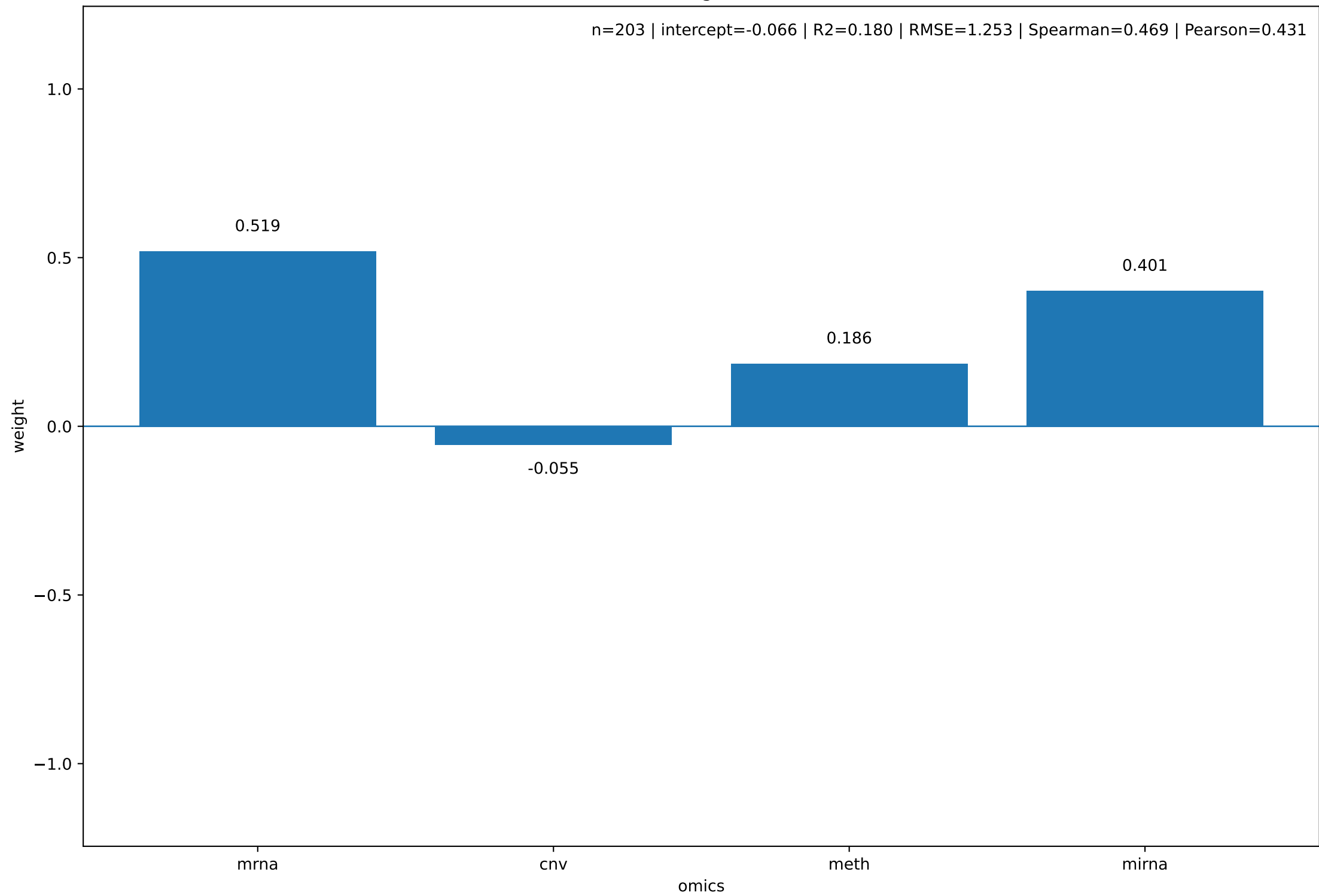
Final omics weights - YK-4-279
