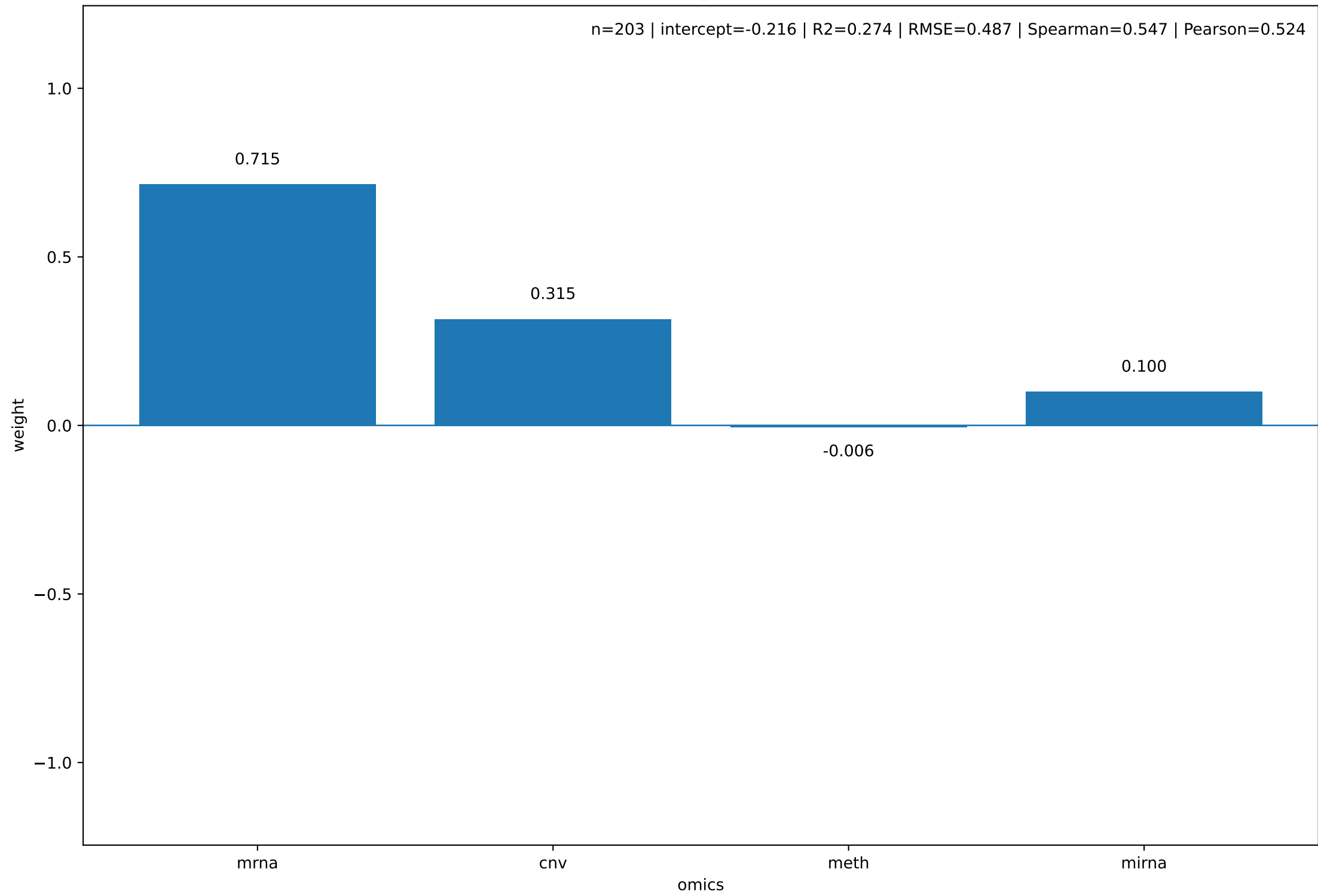
Final omics weights - SGC0946
