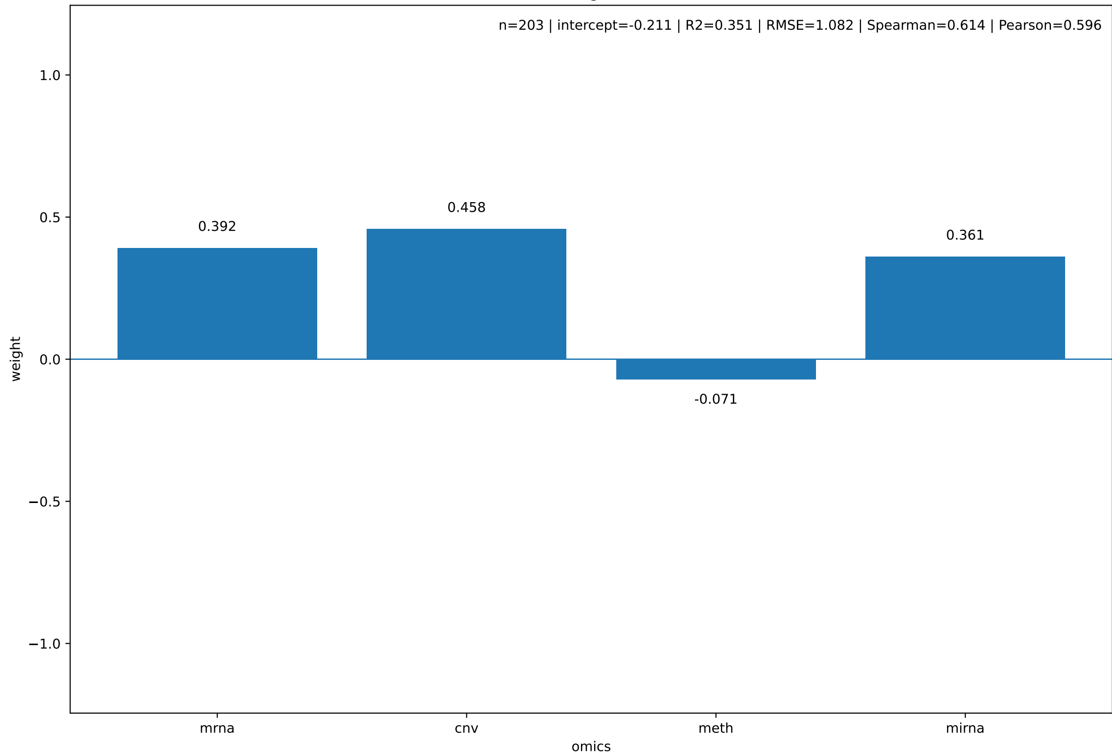
Final omics weights - AZD6738
