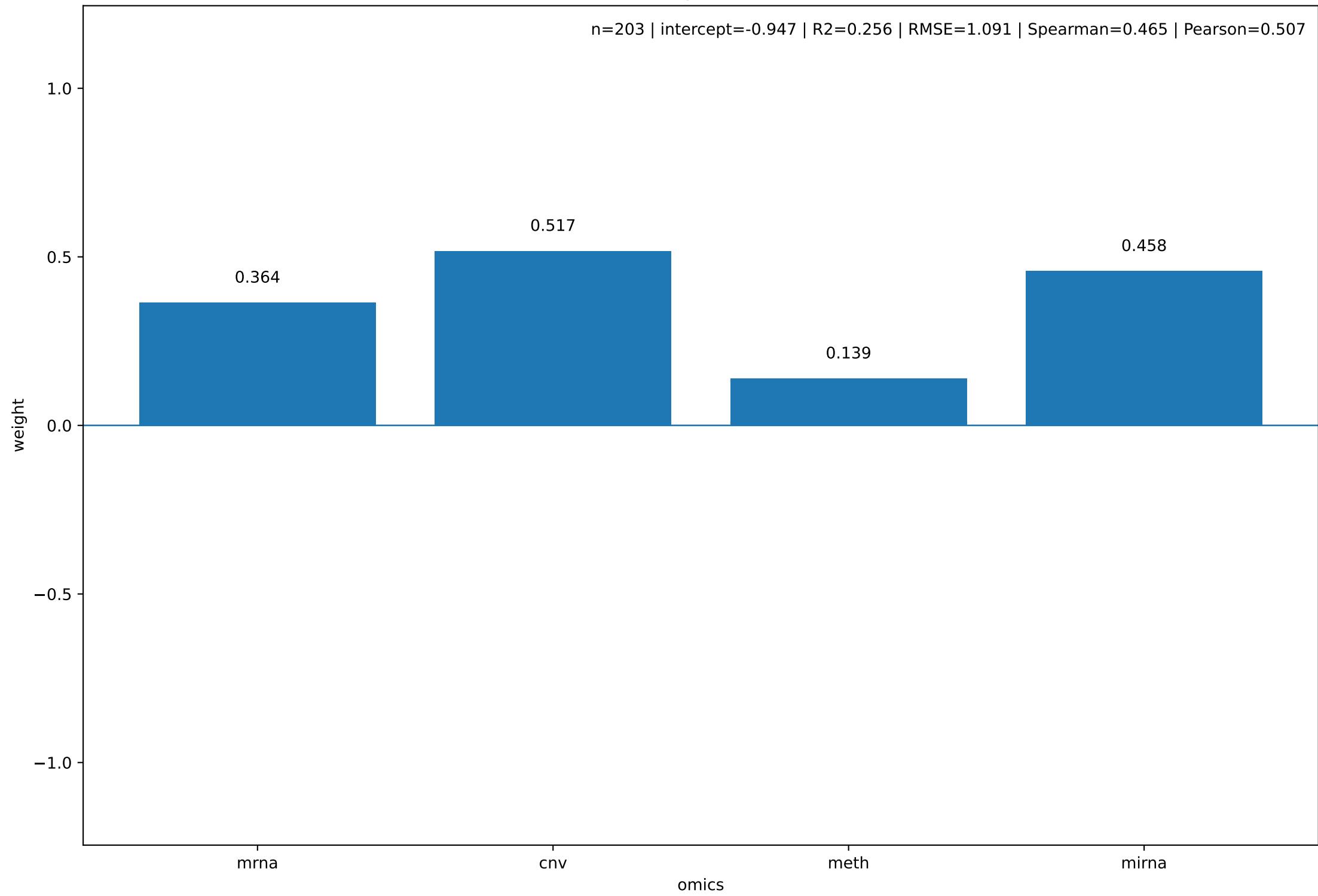
Final omics weights - BMS-536924
