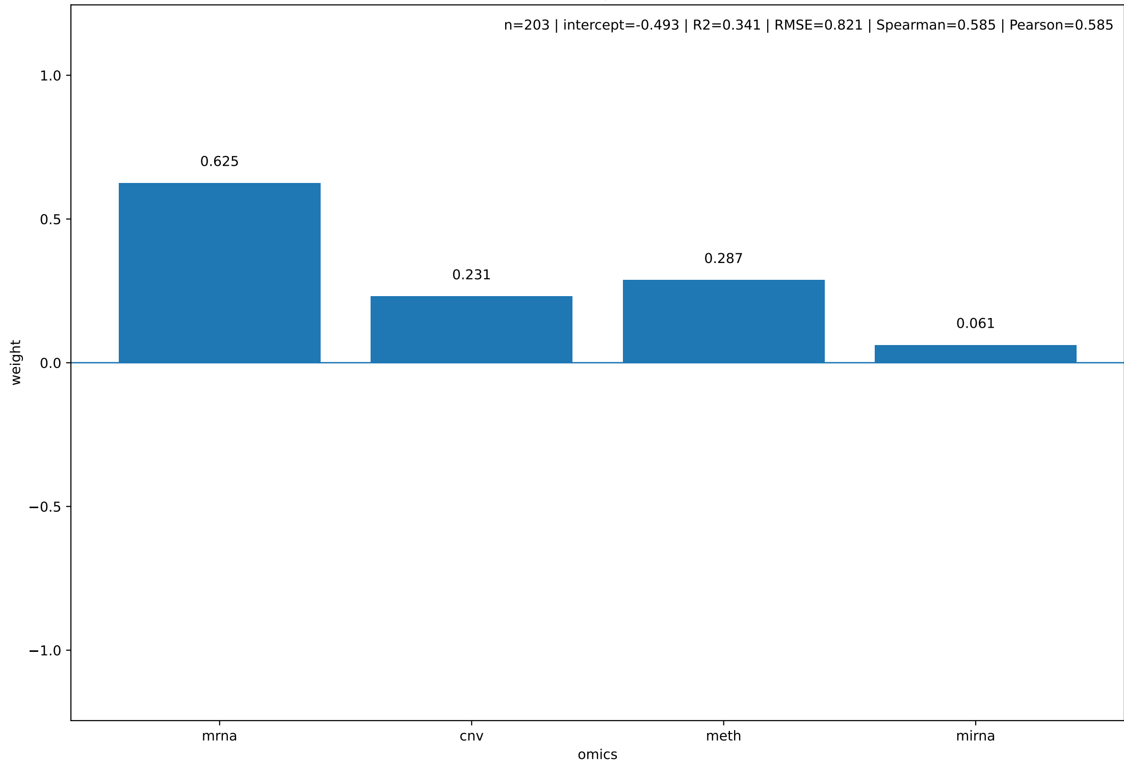
Final omics weights - NU7441
