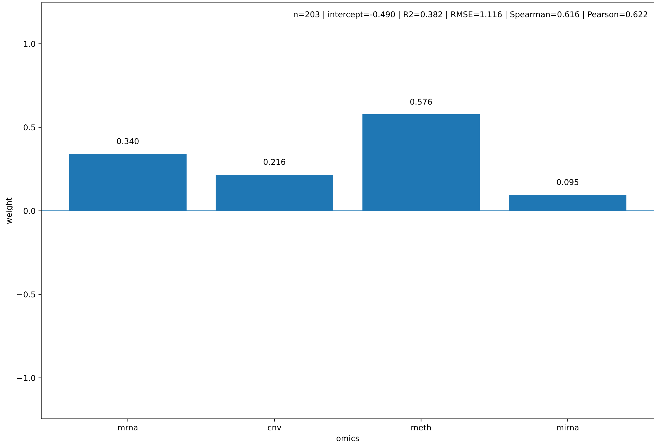
Final omics weights - AXITINIB
