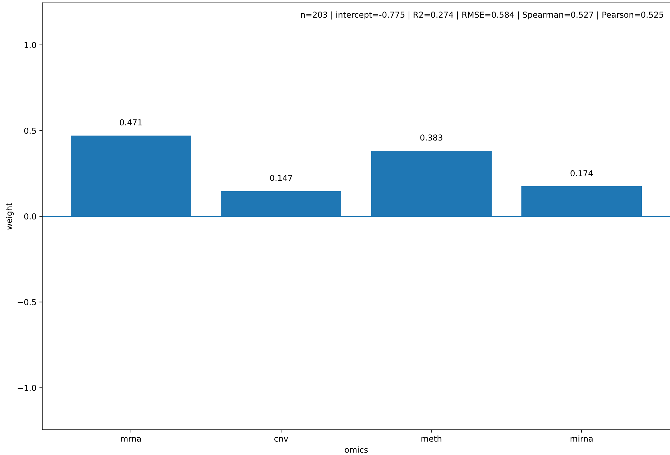
Final omics weights - CCT007093
