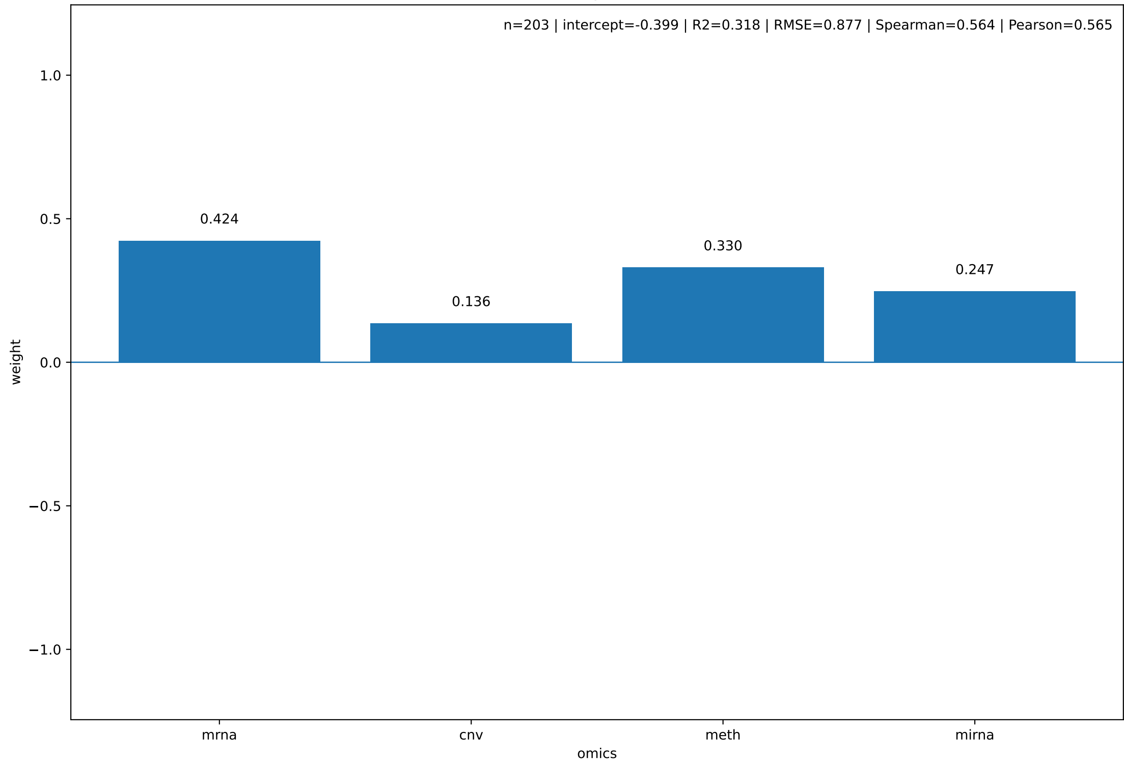
Final omics weights - PD173074
