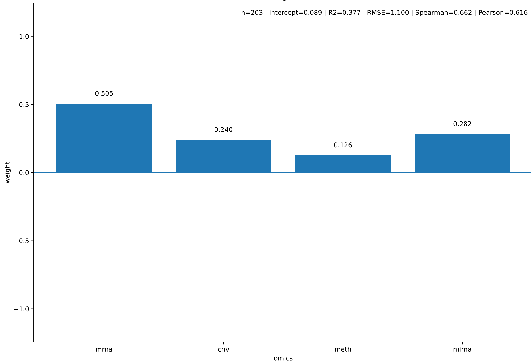
Final omics weights - AZD7762
