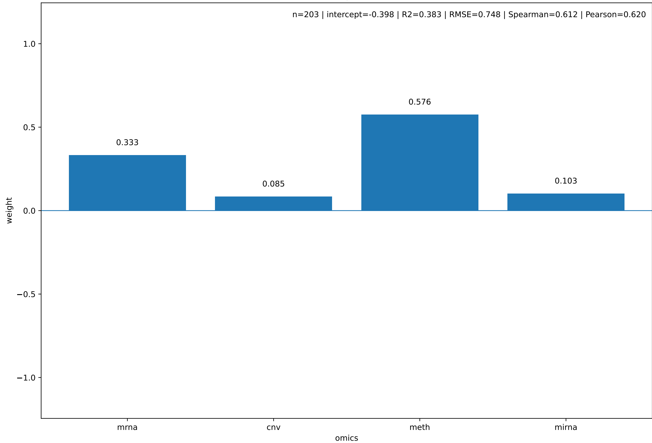
Final omics weights - KU-55933
