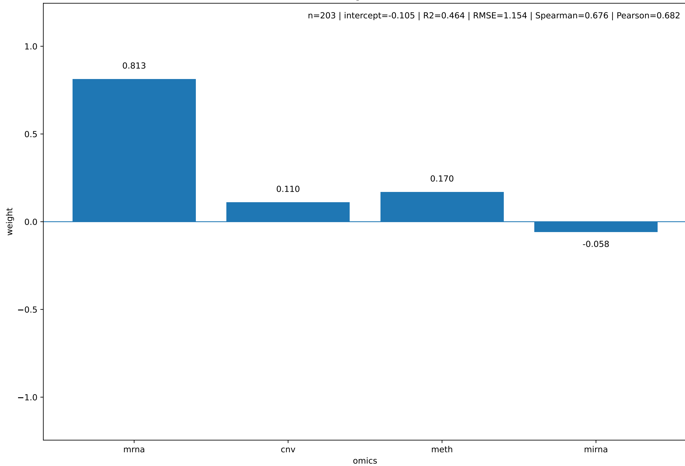
Final omics weights - PALBOCICLIB
