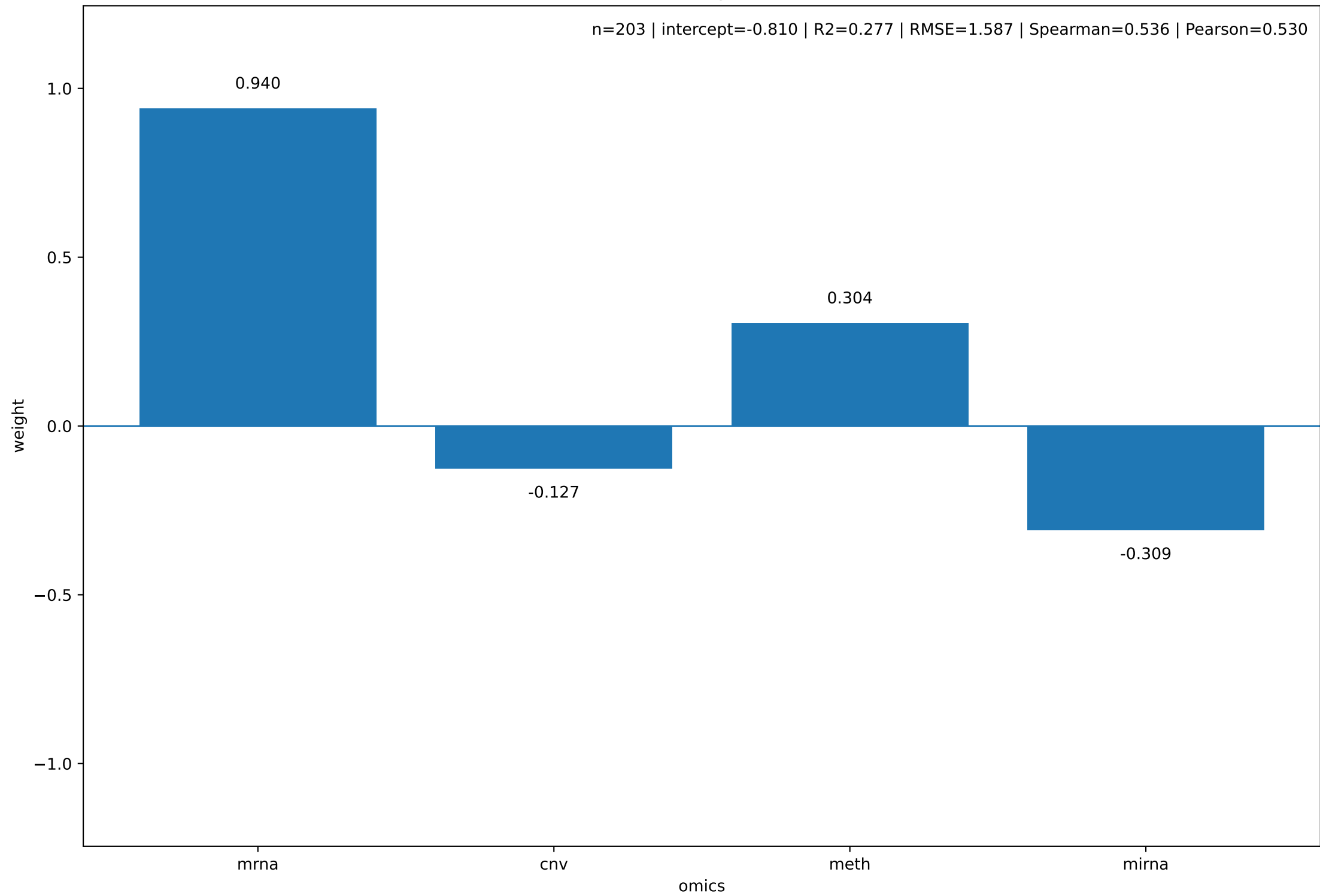
Final omics weights - SN-38
