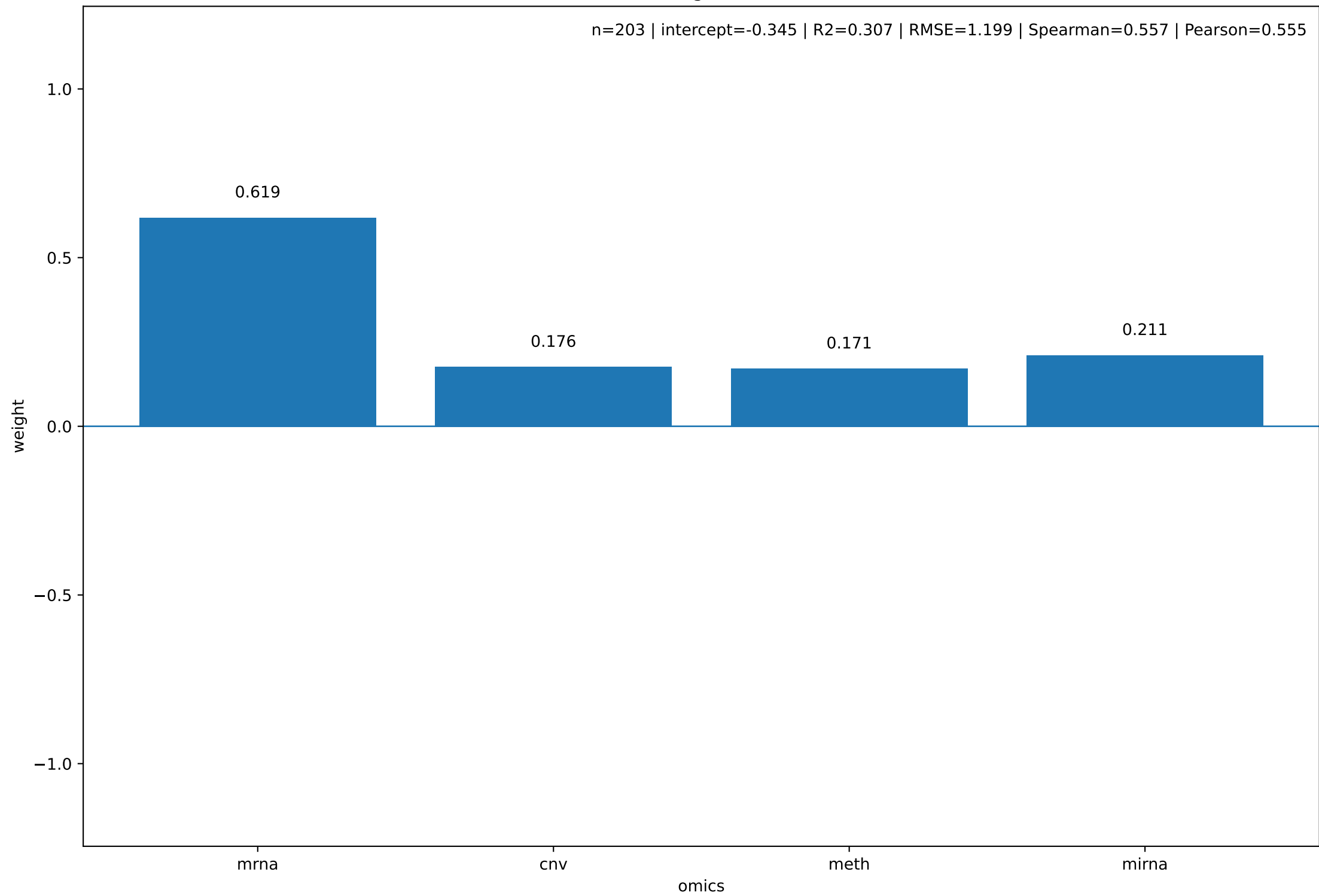
Final omics weights - ZM447439
