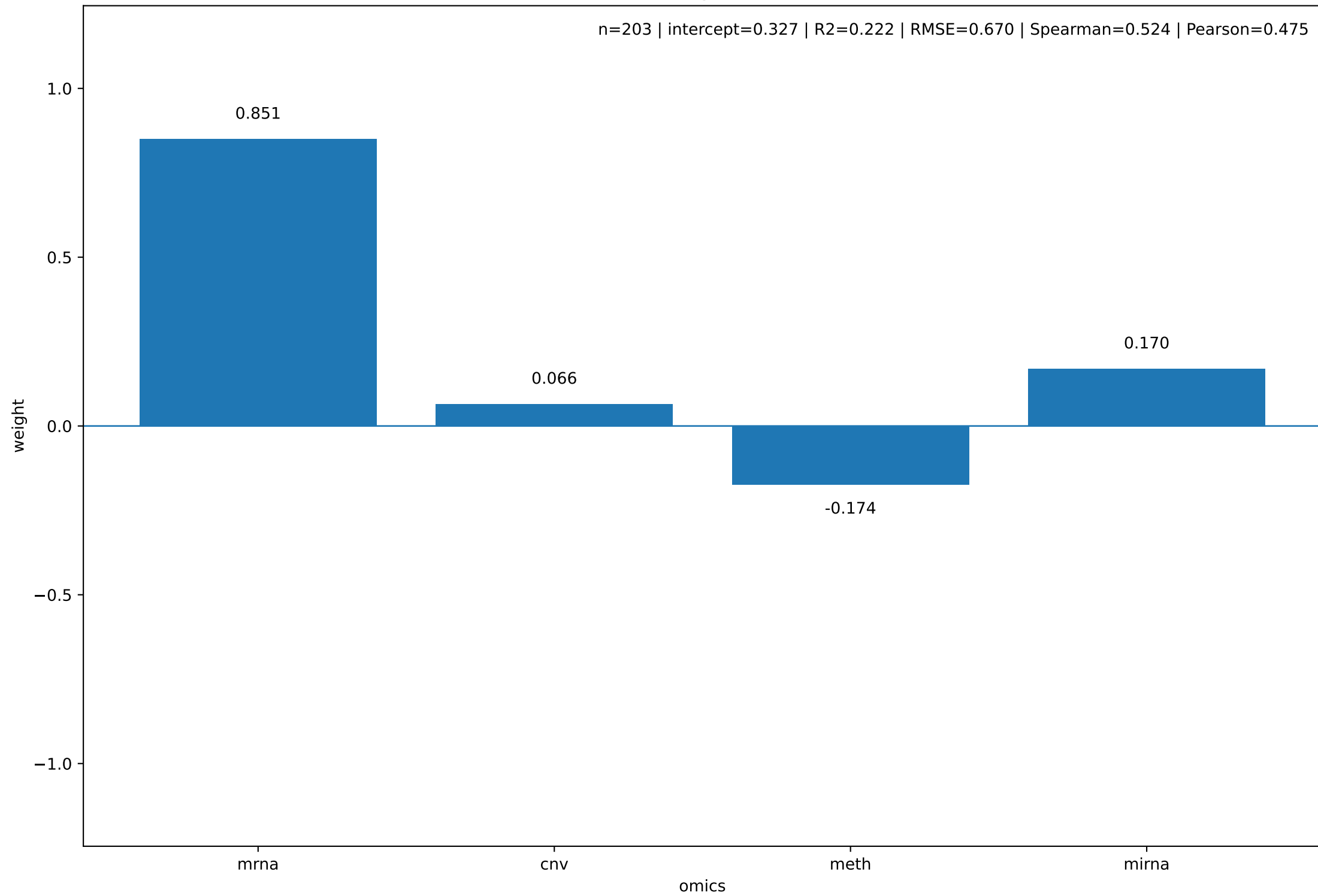
Final omics weights - EHT-1864
