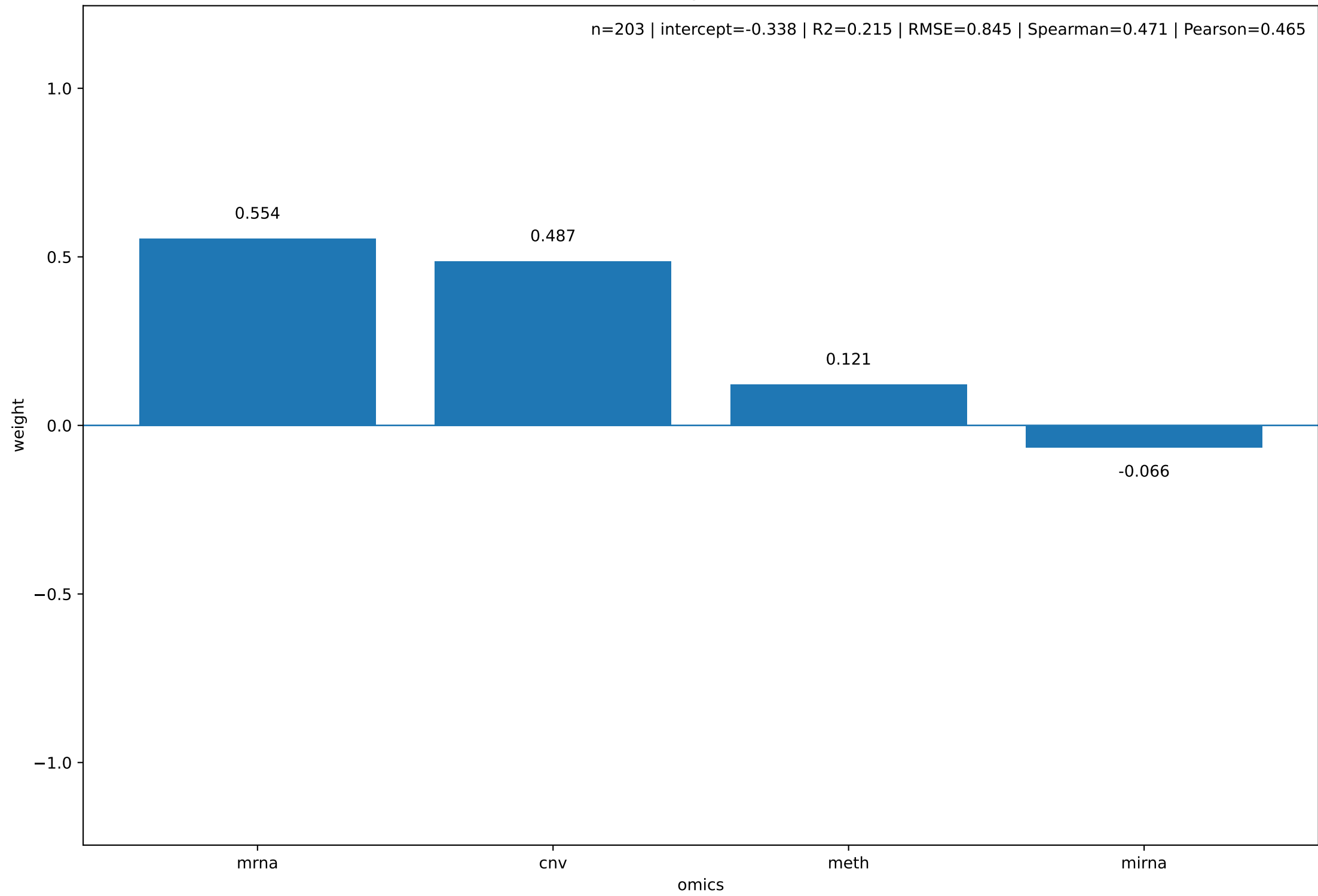
Final omics weights - RUCAPARIB
