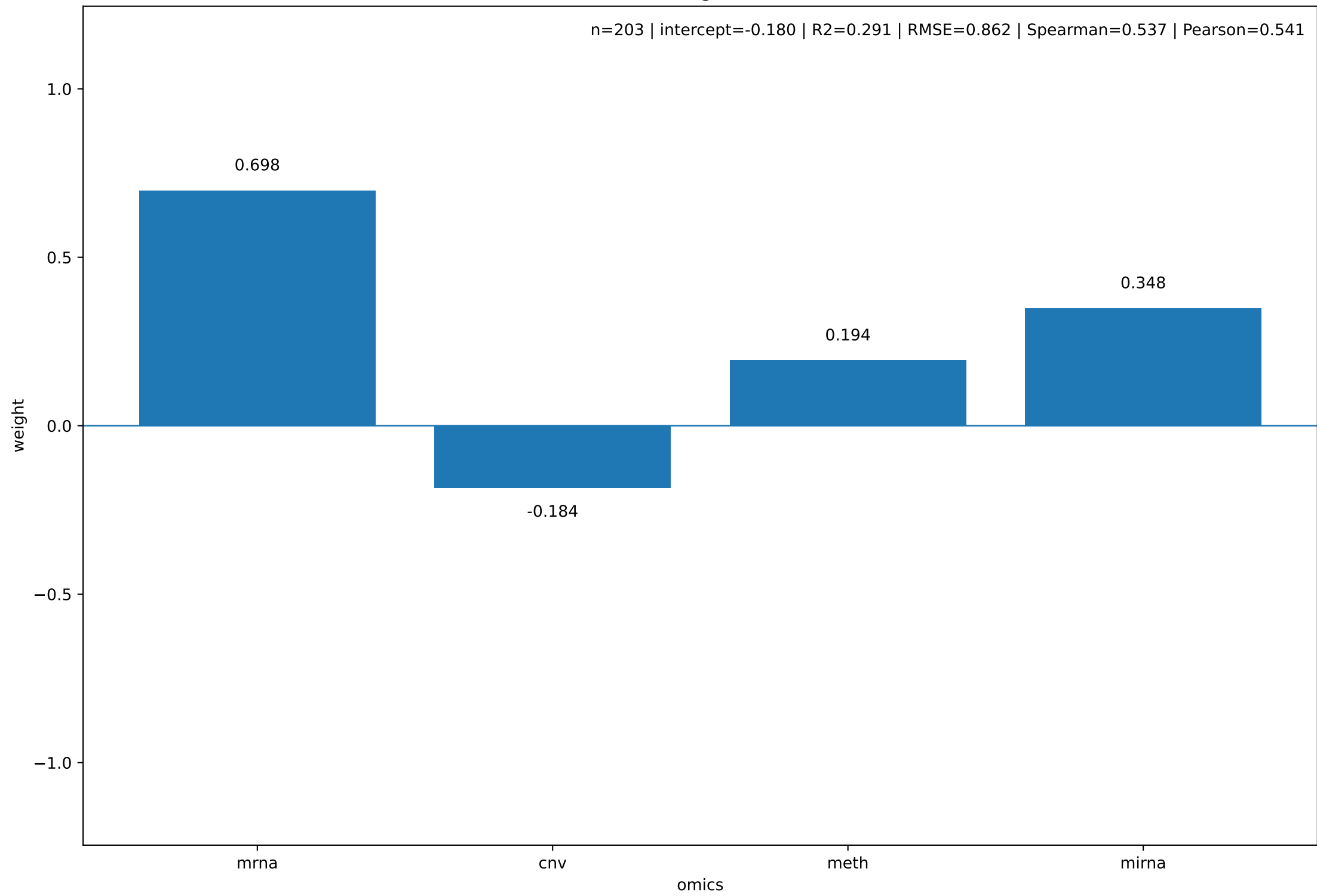
Final omics weights - RO-3306
