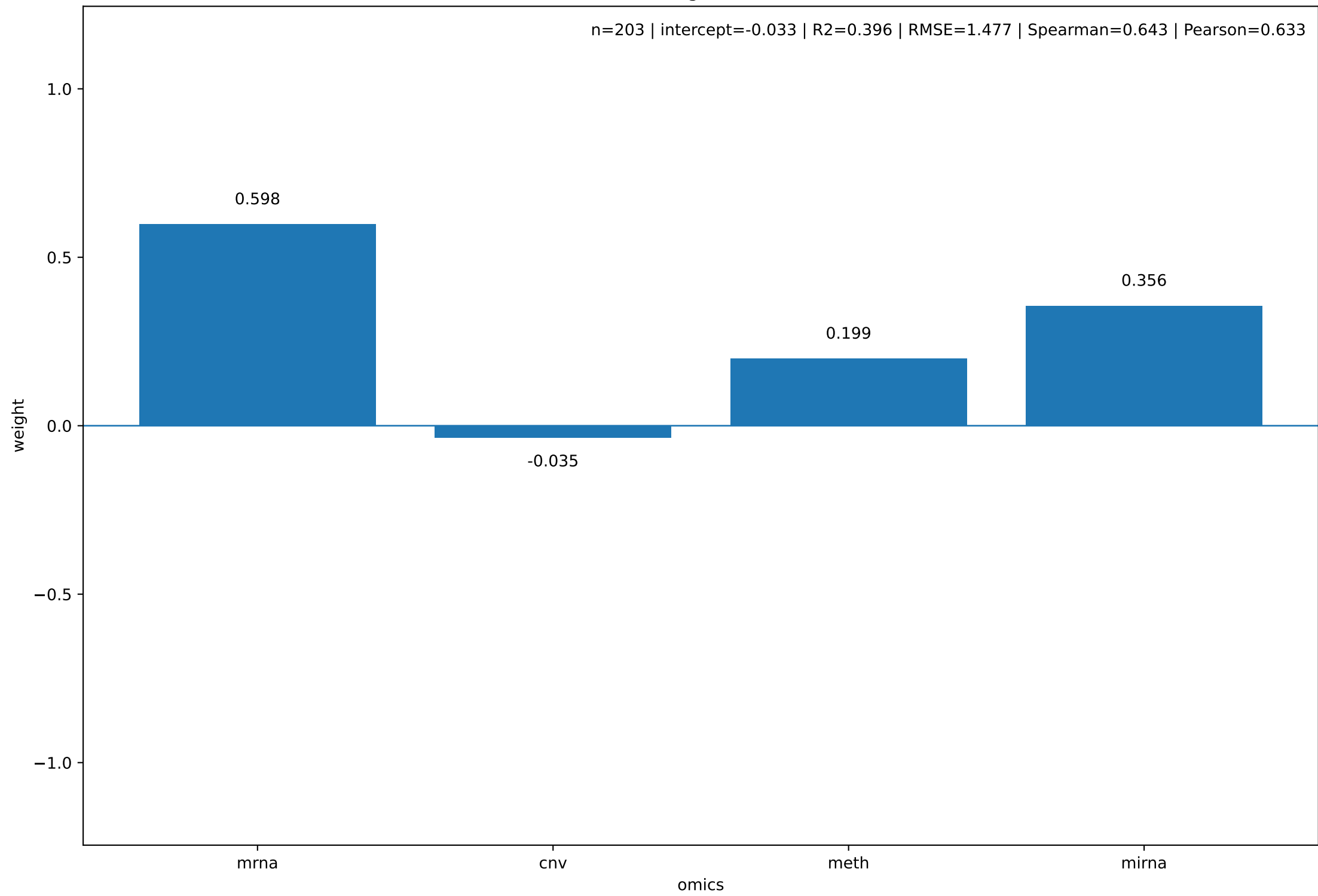
Final omics weights - PD0325901
