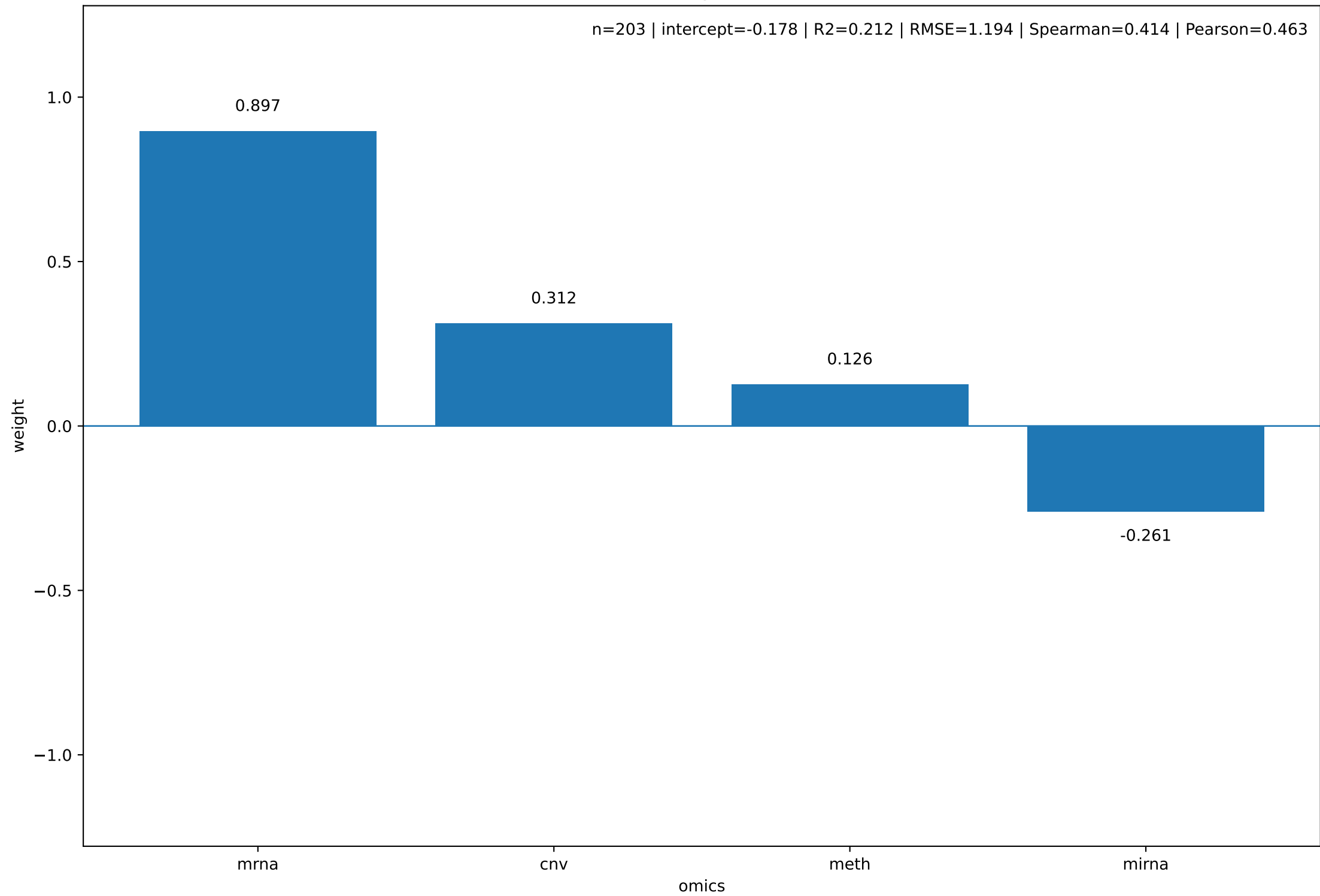
Final omics weights - AZD8186
