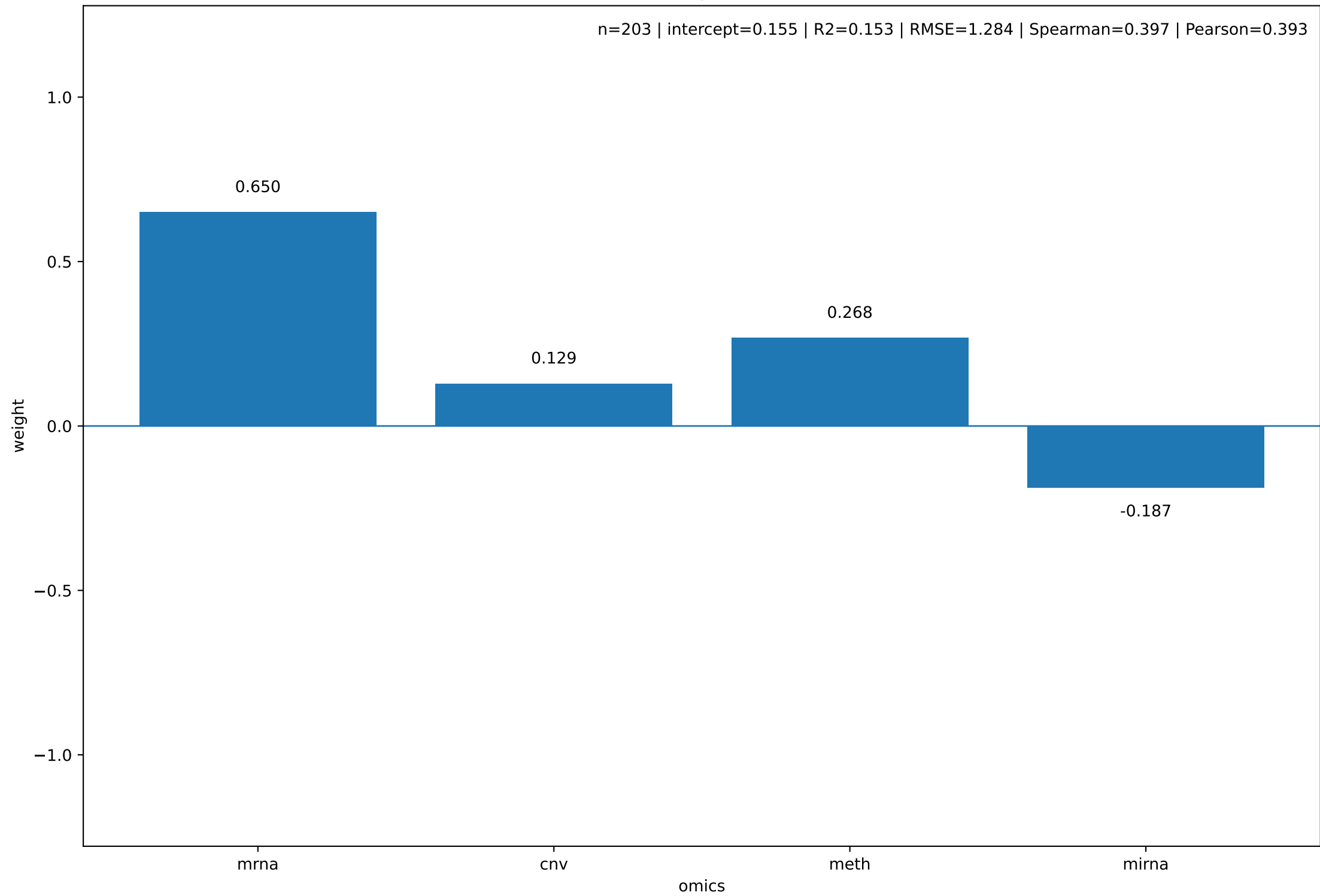
Final omics weights - PICTILISIB
