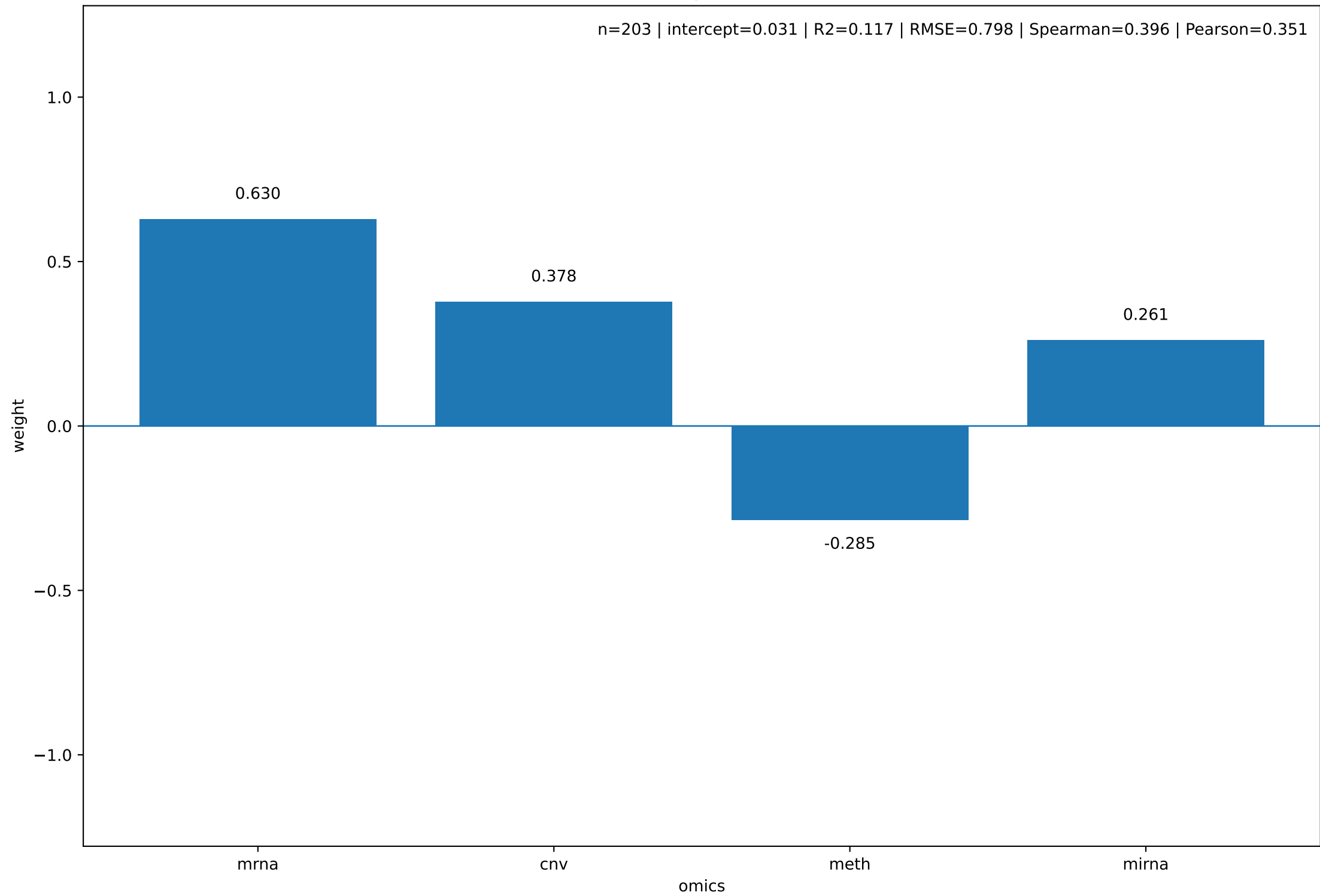
Final omics weights - GW441756
