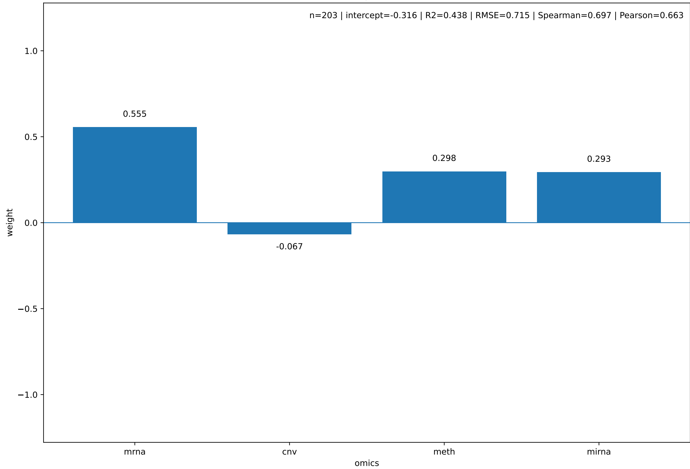
Final omics weights - SB590885
