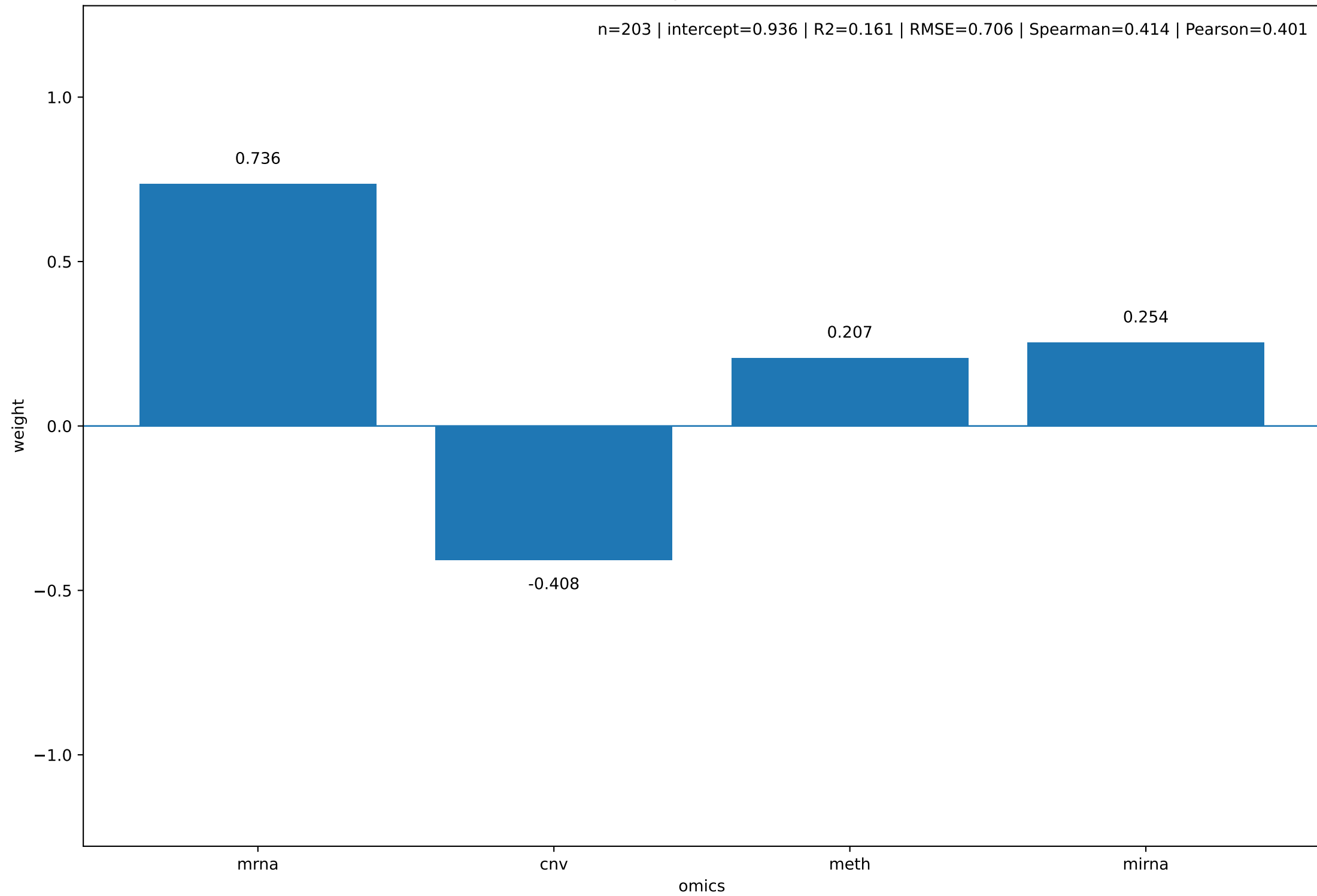
Final omics weights - DORAMAPIMOD
