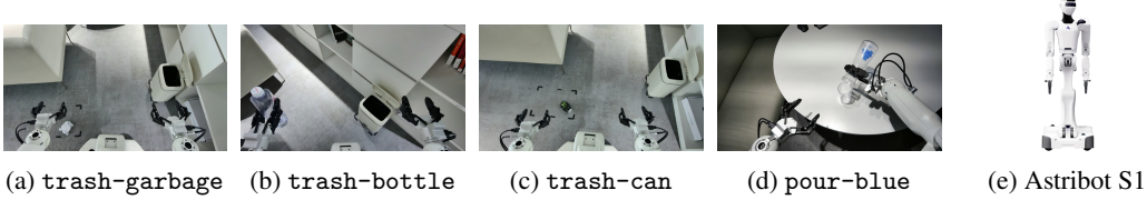
Figure 3: Representative real-robot evaluation scenes and the Astribot S1 platform.
