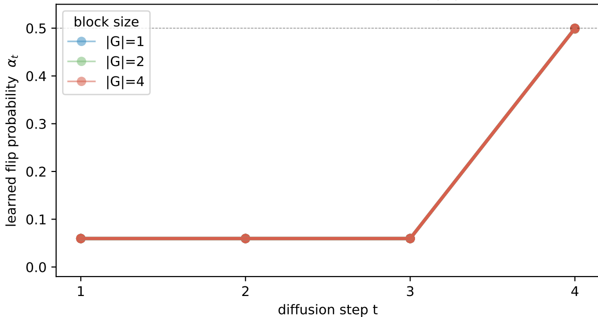
E2: learned forward schedule per run (thin = individual seeds; thick = per- |G| mean)
