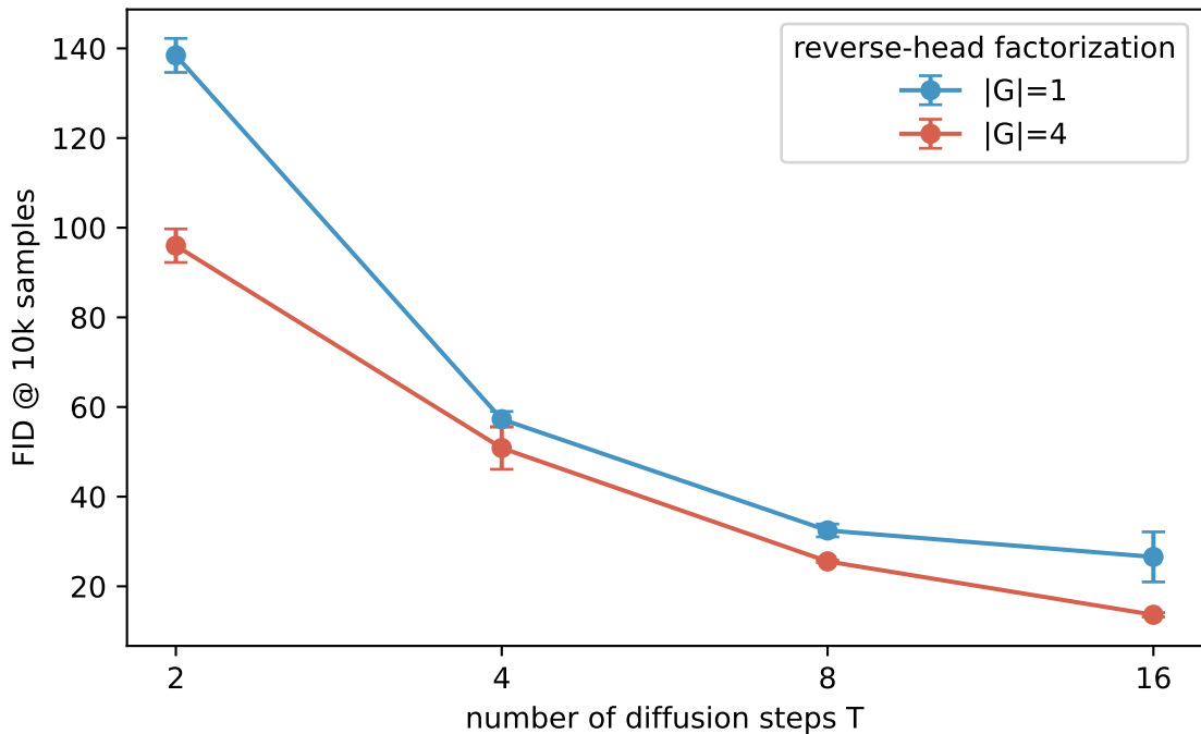
E4: FID vs T (mean \pm std across seeds)
