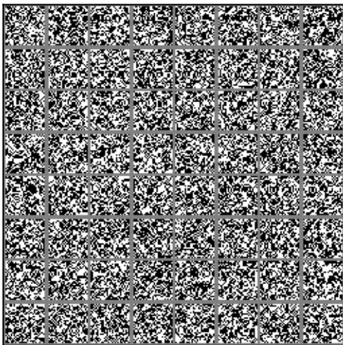
|G|=1 (baseline)
