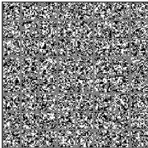
|G|=4 (ours)
