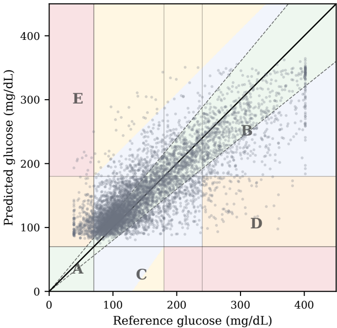
MambaFormer-96, 90 min Zone A=59.29%, Zone A+B=92.76%
