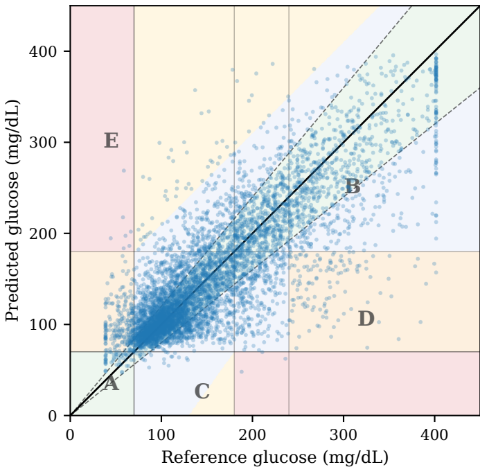
Spectrogram patch-token, 90 min Zone A=64.70%, Zone A+B=93.53%
