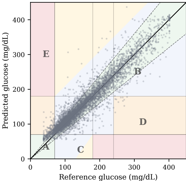
MambaFormer-96 Zone A=87.11%, A+B=97.89%
