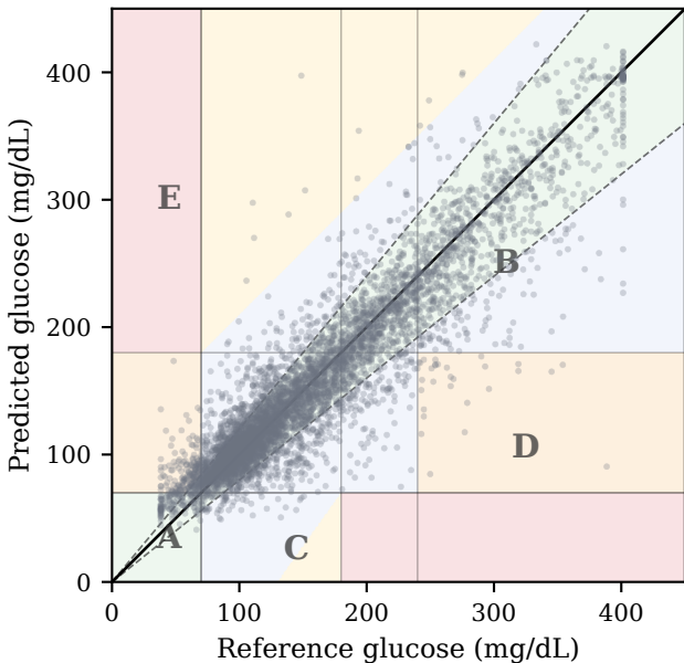
MambaFormer-96 Zone A=80.09%, A+B=97.00%
