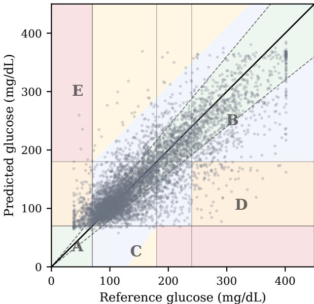
MambaFormer-96 Zone A=68.09%, A+B=93.98%
