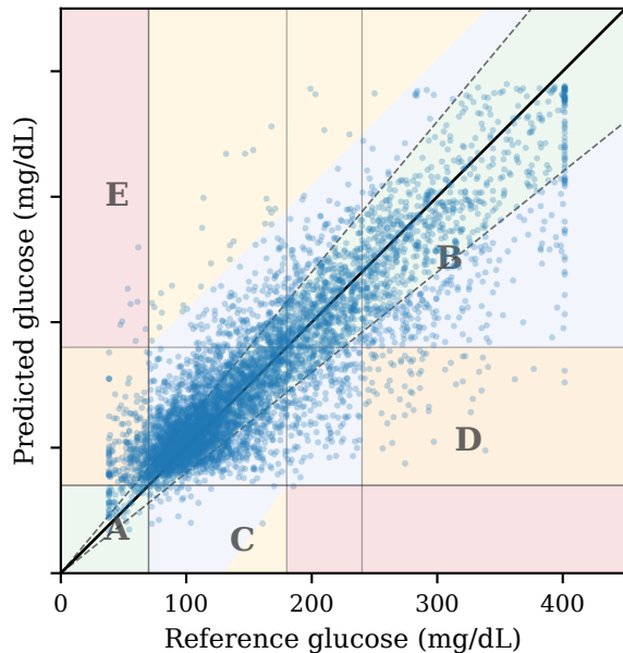
Spectrogram patch-token Zone A=68.16%, A+B=94.56%
