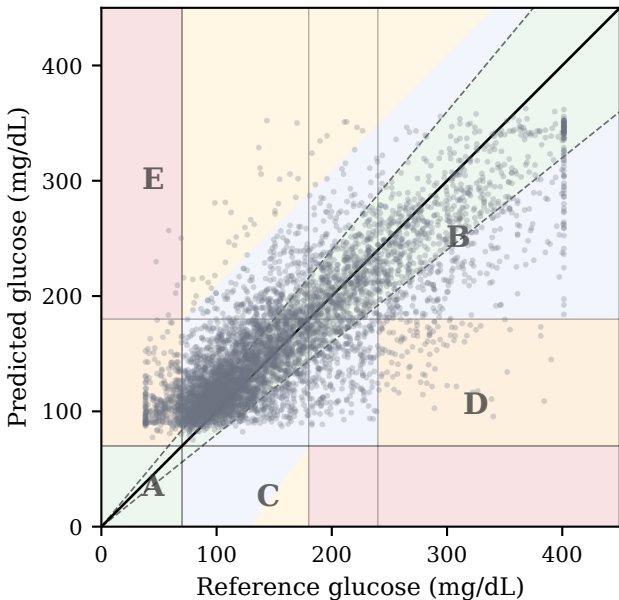
MambaFormer-96 Zone A=59.29%, A+B=92.76%
