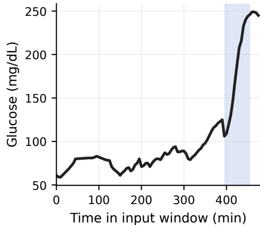
Glucose transition dynamics
