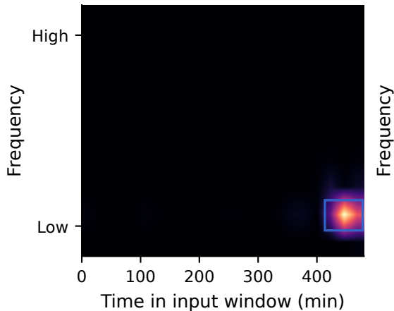
Spectrogram representation
