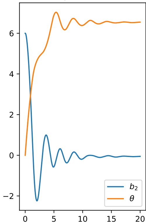
Explicit Euler
