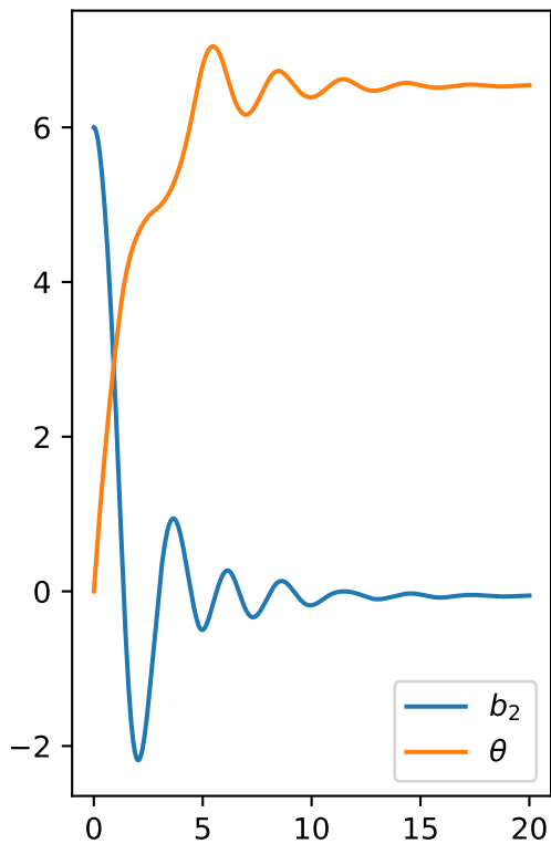
RK4
