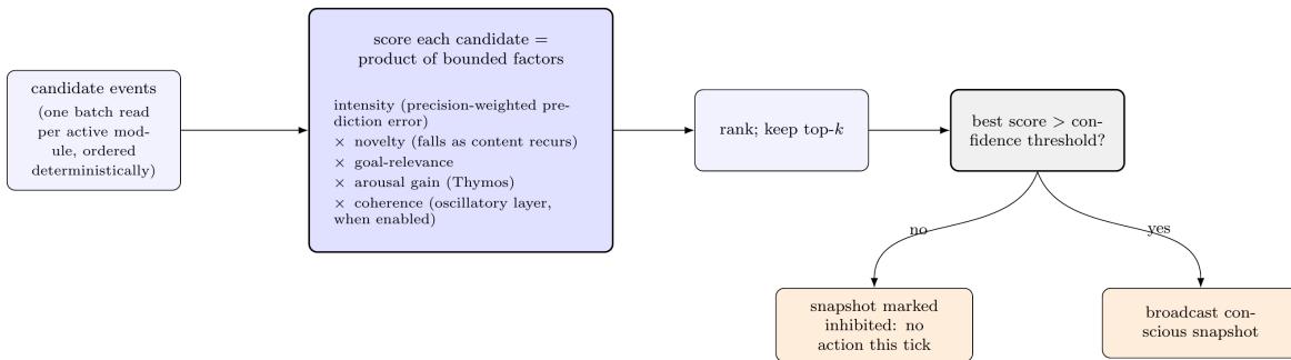
Figure 2: Coalition selection is a deterministic scoring pass, not a graph traversal. Each candidate event is scored as a product of bounded factors; the top-ranked candidates are kept, and when the best score falls below the confidence threshold the whole snapshot is marked inhibited and no action follows on that tick.
