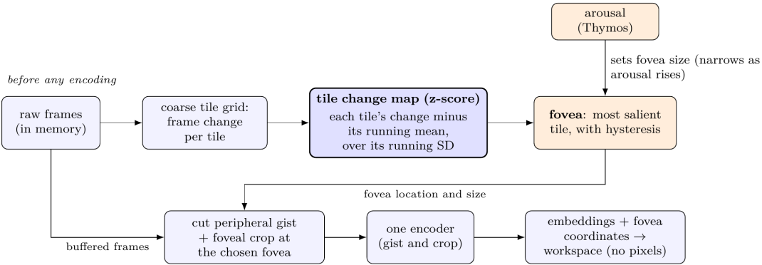
Figure 4: Attention in Topos. Before encoding, a coarse tile change map is computed from the raw frames: each tile’s frame change as a z-score against its own running mean and variance. The fovea moves to the most salient tile, with hysteresis, and arousal sets its size. The peripheral gist and the high-resolution foveal crop are then cut from the buffered frames and pass through one encoder. The embeddings and the fovea’s coordinates reach the workspace, and no pixels do.
