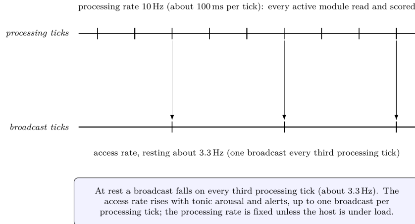
Figure 3: The two rates. Every active module is read and scored at the processing rate (10 Hz), and a broadcast is produced on broadcast ticks at the access rate, shown at its resting value (about 3.3 Hz, one broadcast every third processing tick), which rises with arousal and after alerts.
