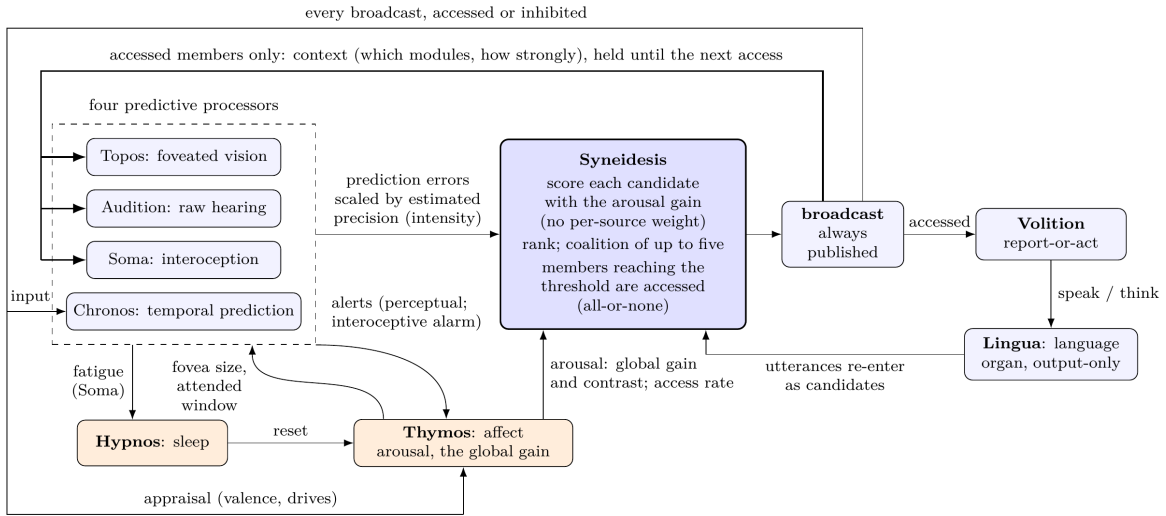
Figure 1: The predictive workspace loop in the base-thesis form. Four predictive processors (foveated vision, raw hearing, interoception, and temporal prediction) report prediction errors scaled by an estimate of their precision. Syneidesis scores the candidates, broadcasts the coalition, and grants access to the members whose scores reach the threshold. A summary of the accessed content becomes the prediction context of Topos, Audition, and Soma, and Chronos takes every broadcast as its input. Thymos appraises every broadcast, and its arousal, raised by the processors' alerts, sets the global gain on selection, the sensory apertures, and the access rate. Hypnos rests the entity on fatigue and resets its affect. Volition reads accessed broadcasts and emits speak or think intents to the output-only language organ Lingua, whose utterances re-enter the competition.
