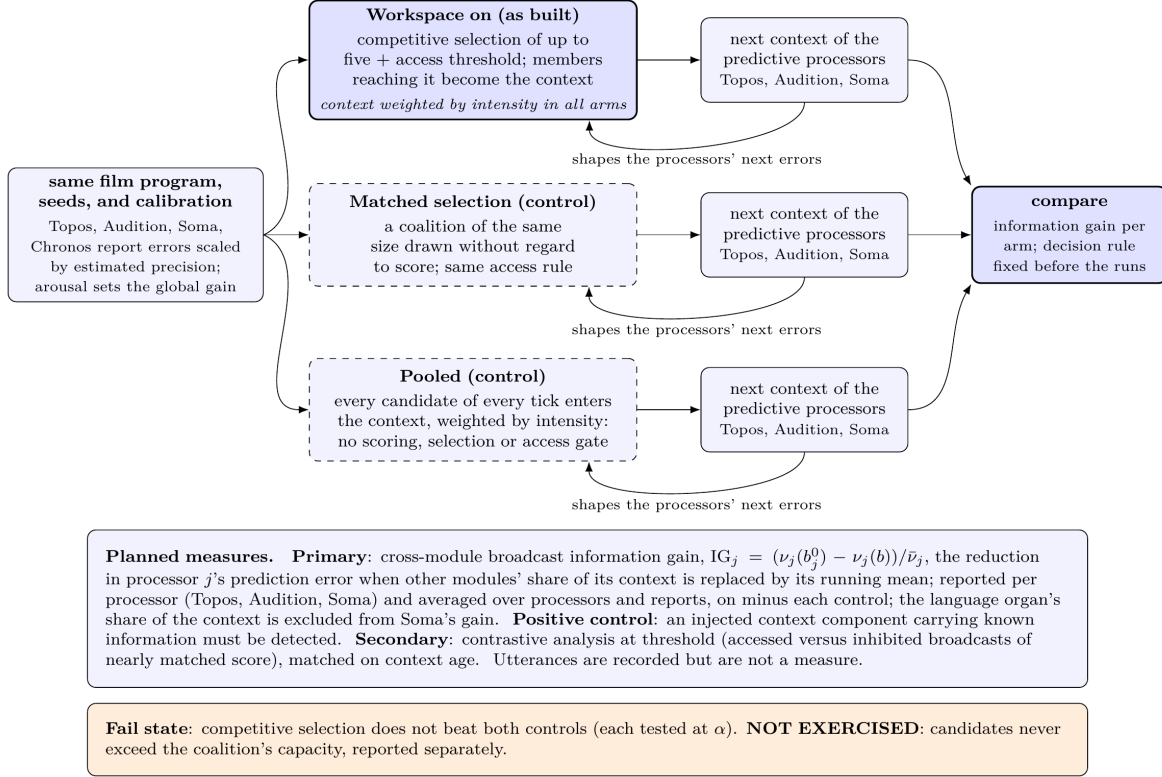
Figure 6: The workspace-mediation ablation. Three arms run on the same film program: competitive selection as built, a matched coalition chosen without regard to score, and the pooled control, in which every candidate enters the context with no selection or access gate. The context is weighted by intensity in all arms and conditions the perceptual and interoceptive processors, and the primary measure is the cross-module information gain, the reduction in each processor's prediction error attributable to other modules' share of that context, reported per processor and averaged. A positive control checks that the measure detects injected information, and the contrastive analysis compares accessed and inhibited broadcasts of nearly matched score, matched on context age. The decision rule is fixed before the runs.
