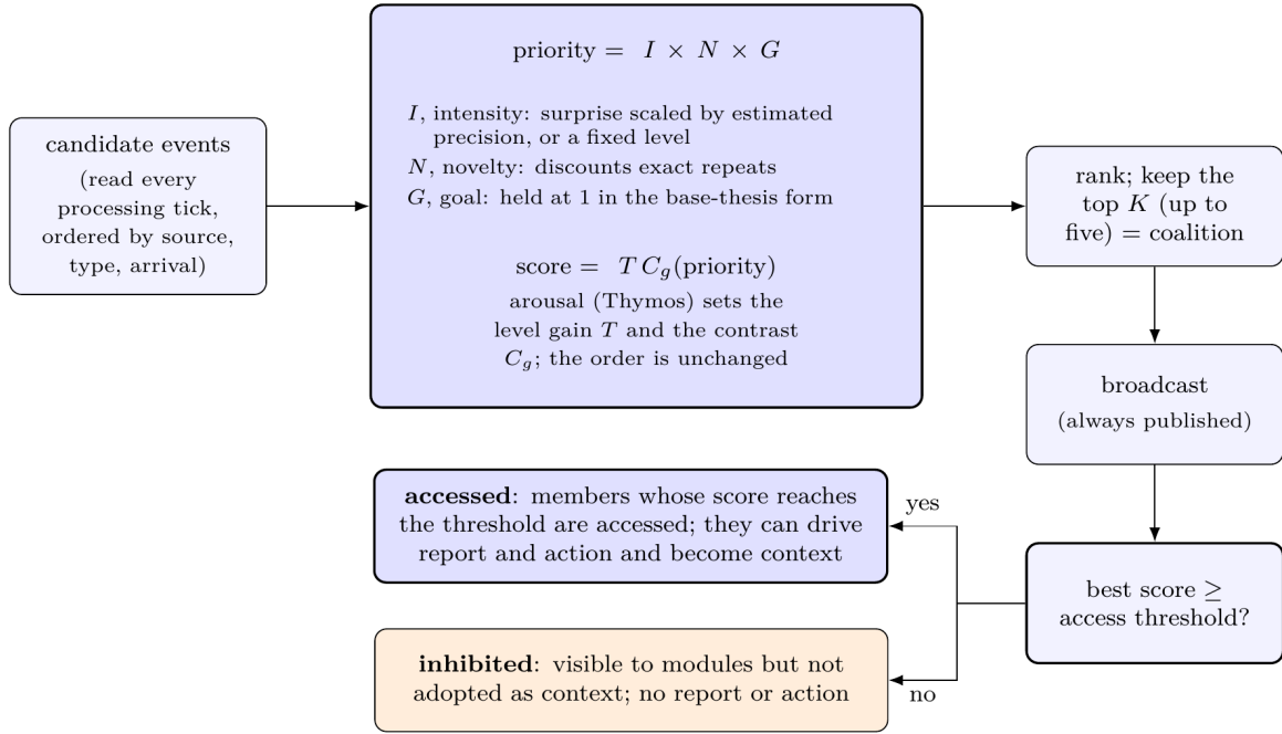
Figure 2: Coalition selection. Each candidate’s priority is the product of its intensity (the producing module’s surprise scaled by its precision, or a fixed level), a novelty factor, and a goal factor held at one. Arousal sets the level and contrast of the score without changing the order, and the top-ranked candidates (up to five) form the coalition, which is always broadcast. Members whose scores reach the access threshold are accessed: they can drive report and action and enter the processors’ prediction context. A broadcast with no accessed member is marked inhibited and stays visible to modules, with no report, action, or change of context.
