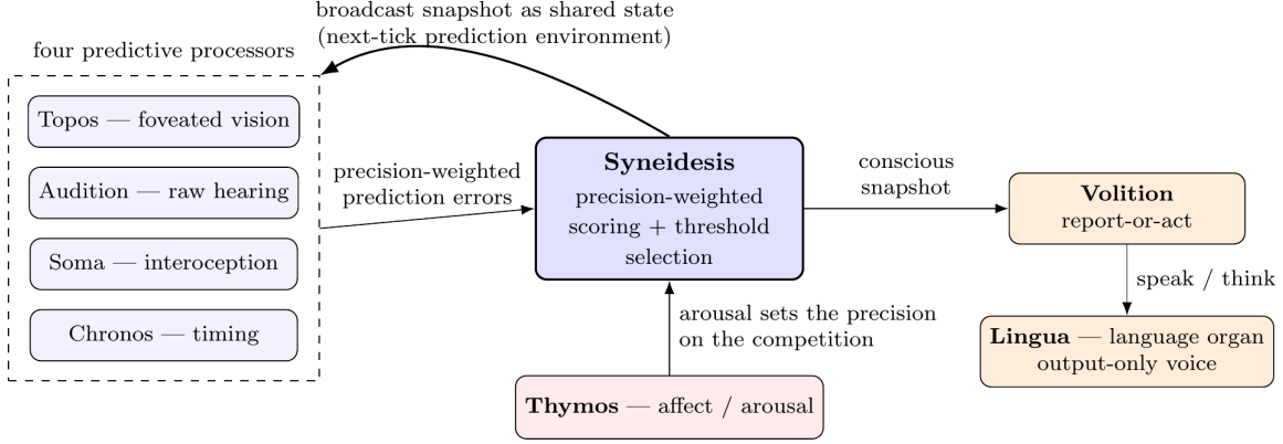
Figure 1: The predictive workspace loop in the base-thesis form. Four predictive processors — foveated vision, raw hearing, interoceptive prediction, and temporal prediction — publish precision-weighted prediction errors into Syneidesis, which scores candidate coalitions and broadcasts the one that crosses the confidence threshold. The broadcast becomes shared state that shapes every module’s prediction environment on the next tick. Thymos sets the precision on the competition through arousal. Volition makes the report-or-act decision; its only outputs are speak and think, verbalized by the output-only language organ Lingua. No real-world effector exists.
