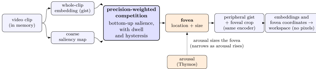
Figure 4: Attention-driven perception in Topos. A whole-clip embedding and a coarse saliency map feed a competition over bottom-up saliency, with dwell and hysteresis. The winner sets the fovea, and arousal sets its size. Peripheral gist and the high-resolution foveal crop share one encoder. The peripheral and foveal embeddings and the fovea’s coordinates reach the workspace, while no pixels do.
