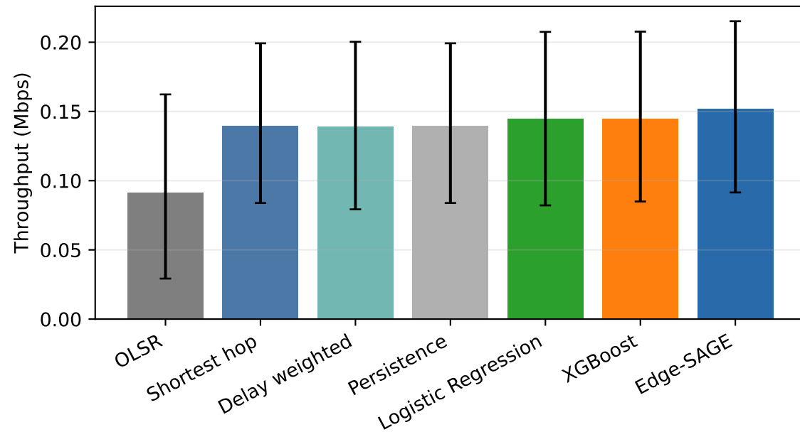
Throughput (Mbps) (higher is better)
