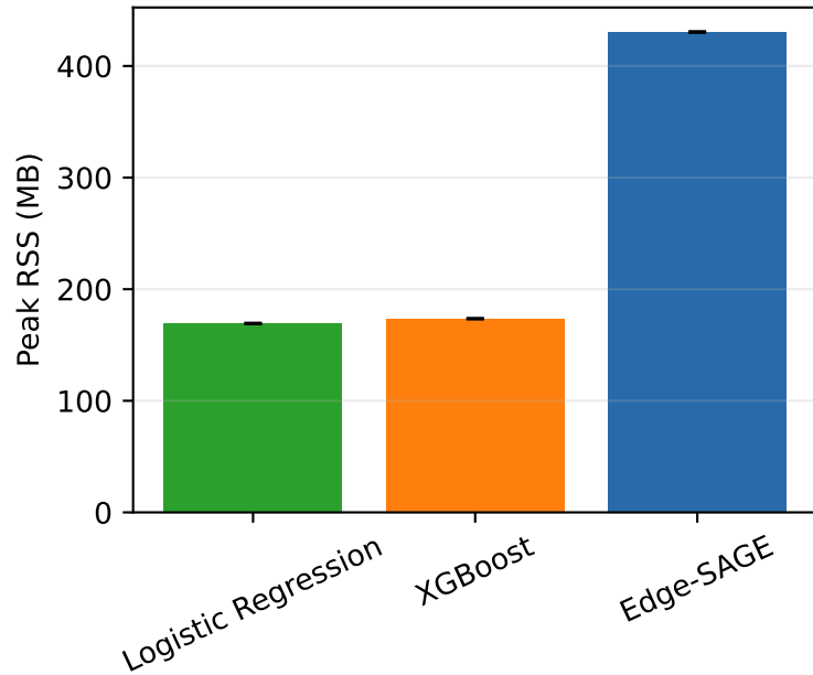
CPU inference cost (survival, k=3, one thread)
