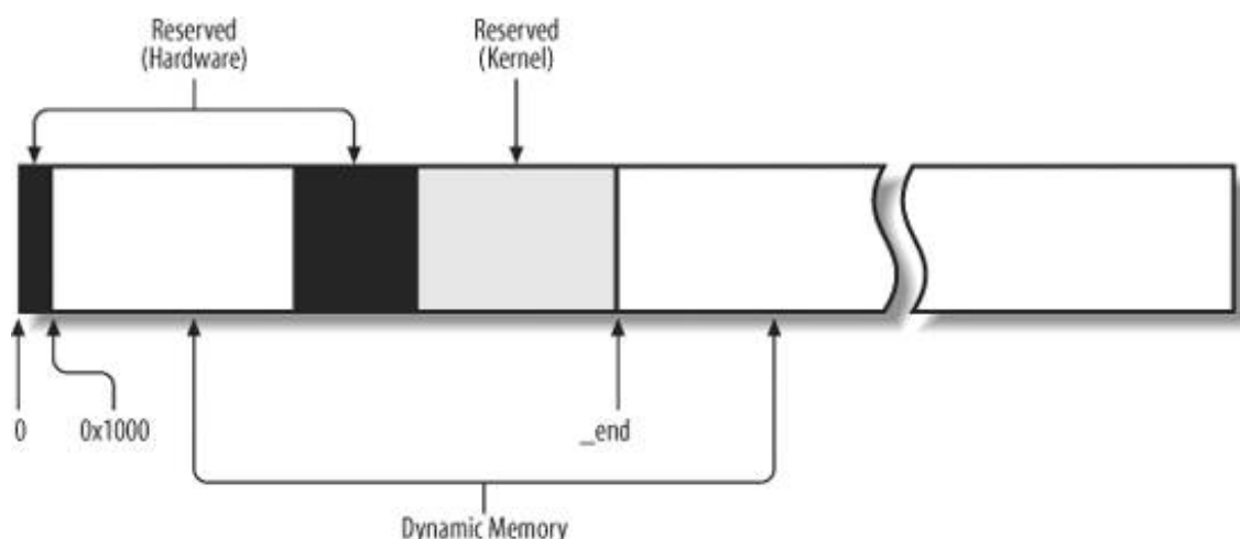
Figure 8-1. Dynamic memory
