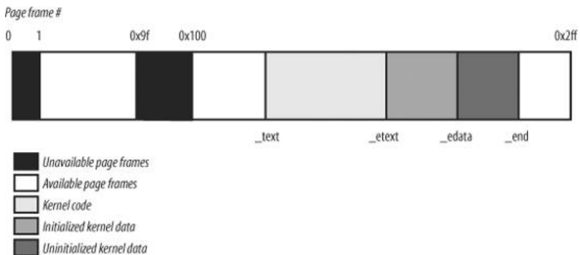
Figure 2-13. The first 768 page frames (3 MB) in Linux 2.6
