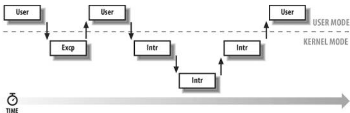
Figure 1-3. Interleaving of kernel control paths
