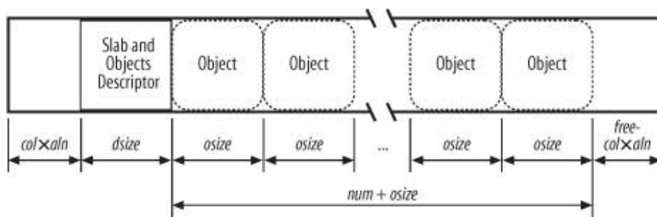
Figure 8-6. Slab with color col and alignment aln
