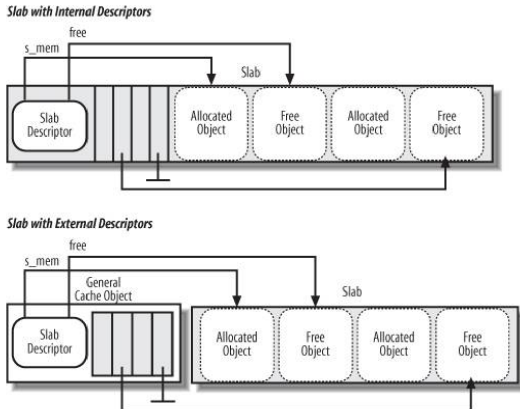
Figure 8-5. Relationships between slab and object descriptors
