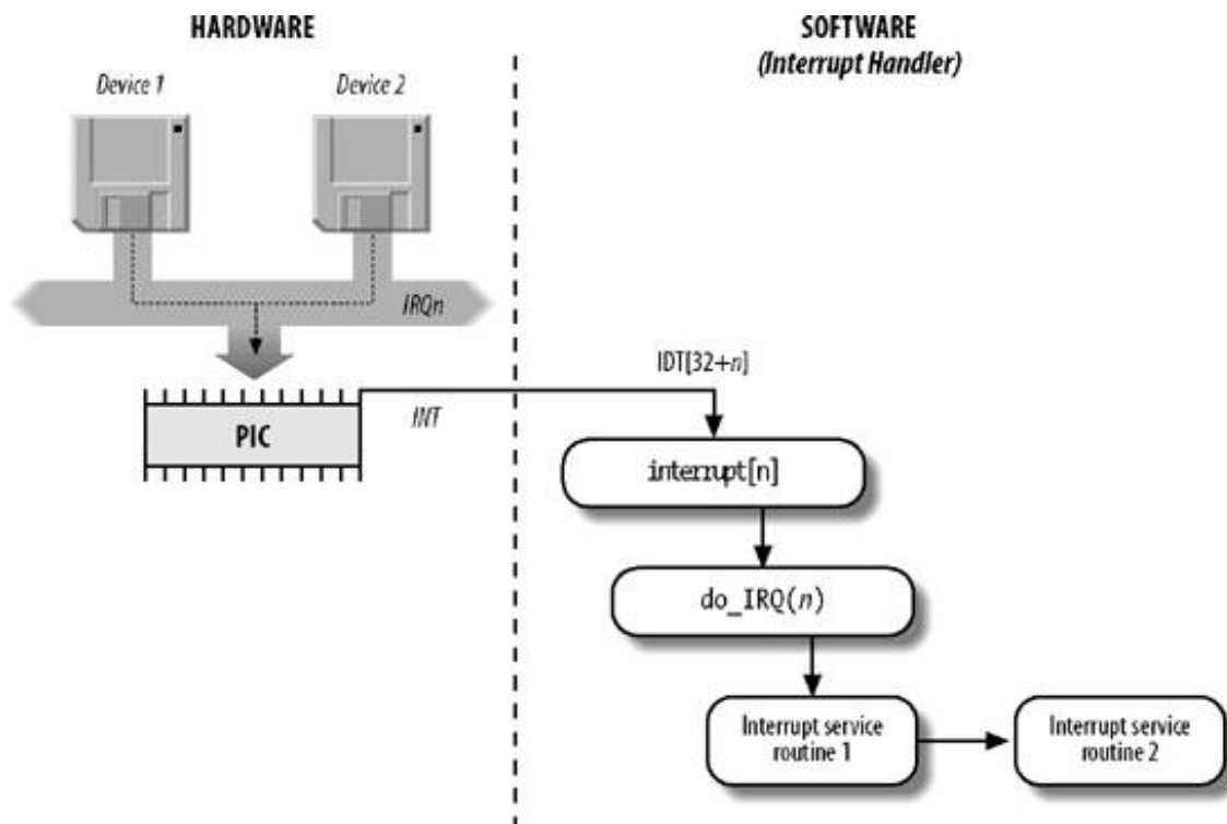
Figure 4-4. I/O interrupt handling
