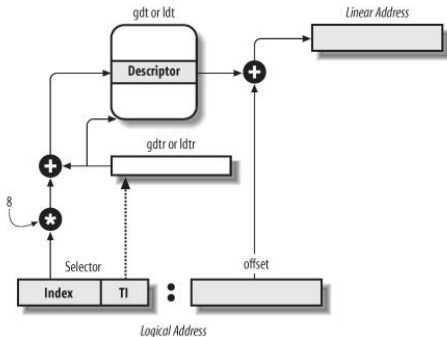
Figure 2-5. Translating a logical address
