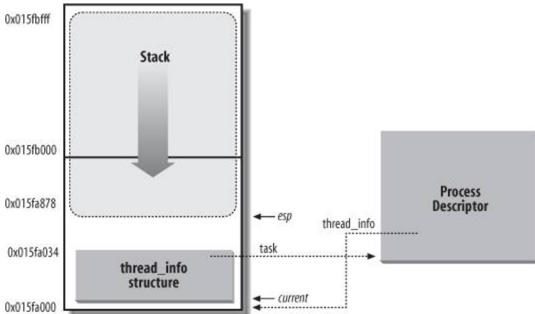
Figure 3-2. Storing the thread_info structure and the process kernel stack in two page frames
