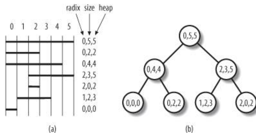
Figure 17-2. A simple example of priority search tree
