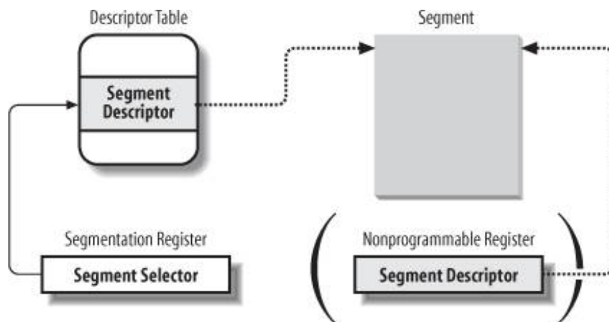
Figure 2-4. Segment Selector and Segment Descriptor
