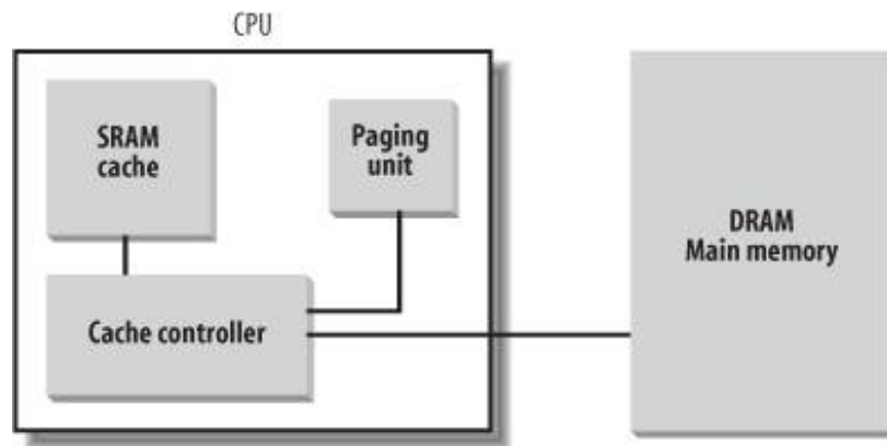
Figure 2-10. Processor hardware cache
