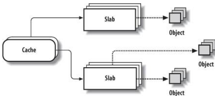
Figure 8-3. The slab allocator components
