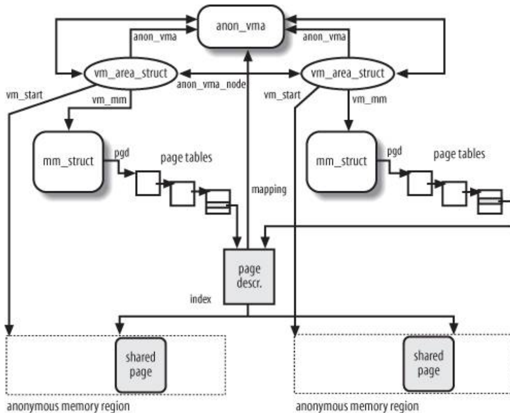
Figure 17-1. Object-based reverse mapping for anonymous pages
