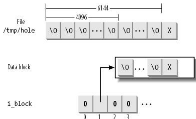
Figure 18-6. A file with an initial hole
