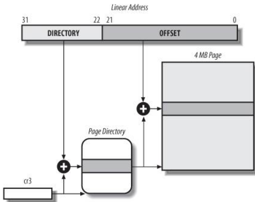
Figure 2-8. Extended paging
