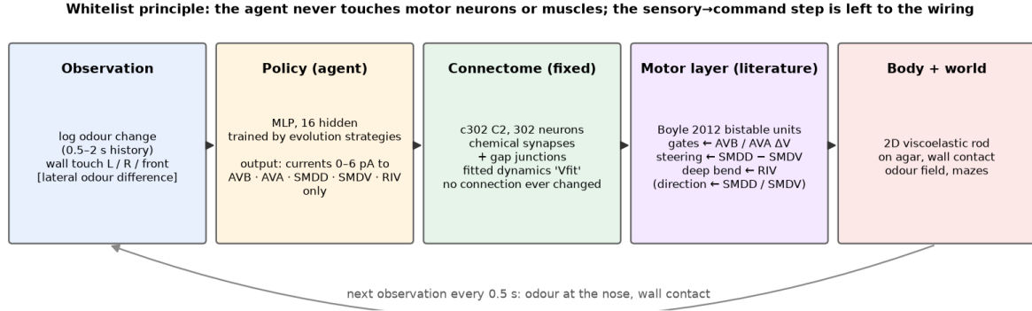
Figure 1: The pipeline and the whitelist principle. Observation → policy → stimulation of whitelisted interneurons → fixed c302 connectome with fitted dynamics → literature motor layer → viscoelastic body in an odour field with walls.
