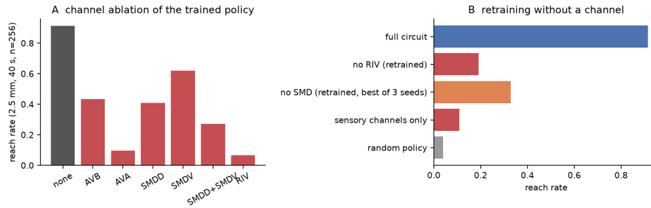
Figure 3: The minimal circuit. Reach rate after masking each channel of the trained policy, and after retraining without RIV or without steering.
