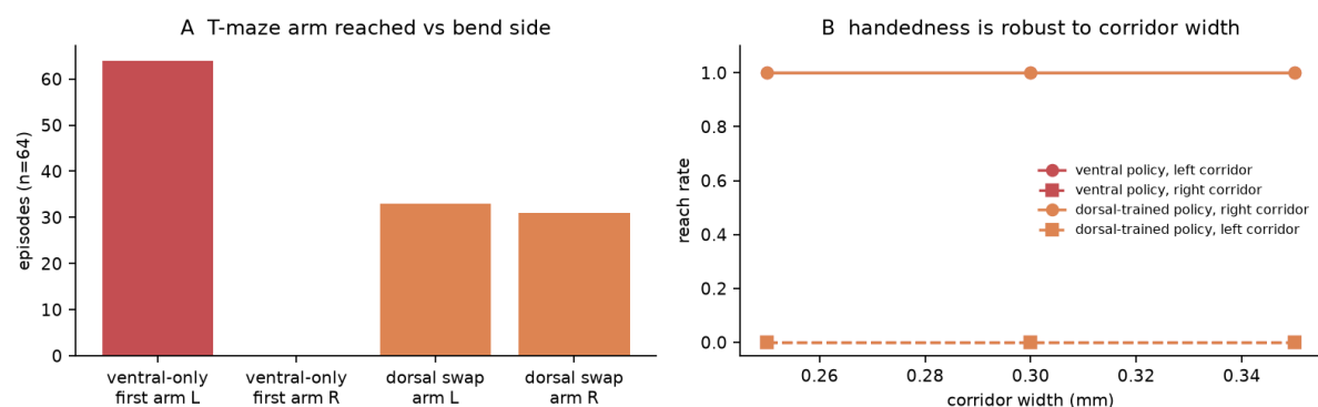
Figure 5: Bend direction is turn direction. Left- and right-turn corridors under the ventral-only and SMD-direction rules across corridor widths, and the dorsal-swap control.
