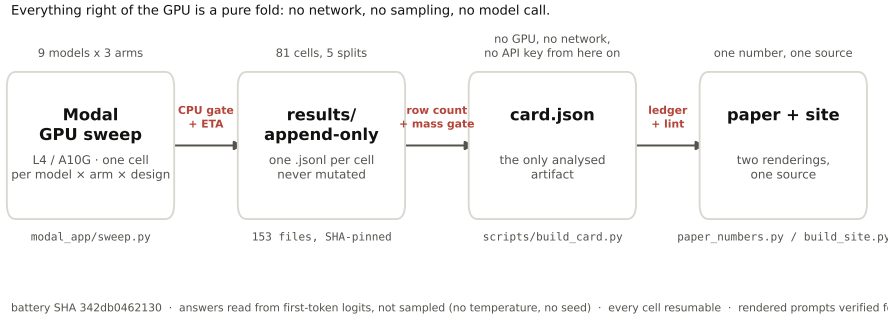
Figure 1: The measurement pipeline. A rented GPU is the only stage that calls a model; everything to its right is a pure fold over files on disk, with no network, no sampling and no API key. Answers are read from the first-token logit distribution rather than sampled, so temperature, top- p and seed are absent from the design. Each arrow carries the gate that guards it: a CPU-only dry run of the whole battery before any GPU is rented, a row-count and answer-mass check before a cell may enter card.json , and a claims-ledger and lint check before any number reaches prose. Because the paper and the public results page are two renderings of the same card.json , they cannot disagree.
