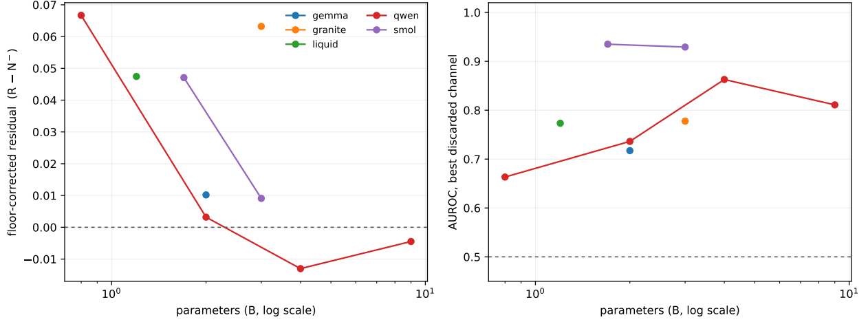
Figure 4: The metric’s residual falls with size; the channel it throws away does not. Left: floor-corrected residual against parameter count, one line per family, log x-axis, dashed line at zero. Right: AUROC of the best discarded channel, dashed line at chance. Single-model families appear as single points. The two panels are drawn together because either alone misleads — the left would read as “nothing here at scale”, and the right as a detector result rather than as evidence about what the metric declines to use.
