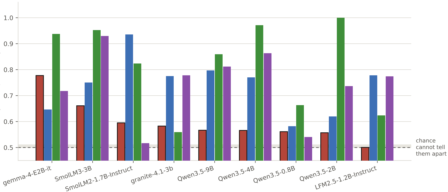
separation of real vs invented outcomes (AUROC, oriented)
