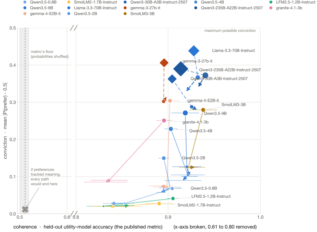
Figure 2: Every model is a path, not a point. Each trajectory starts on real outcomes, moves to invented outcomes with magnitudes kept, and ends at invented outcomes with magnitudes removed. If the metric tracked meaning the paths would run down- and-left . They run almost straight down: conviction falls away while the metric barely registers it. Both axes span their full operating range, so the steepness is the data’s and not a choice of zoom.
