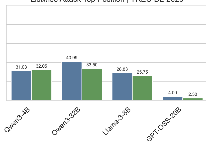
Listwise Attack Top Position | TREC-DL-2020
