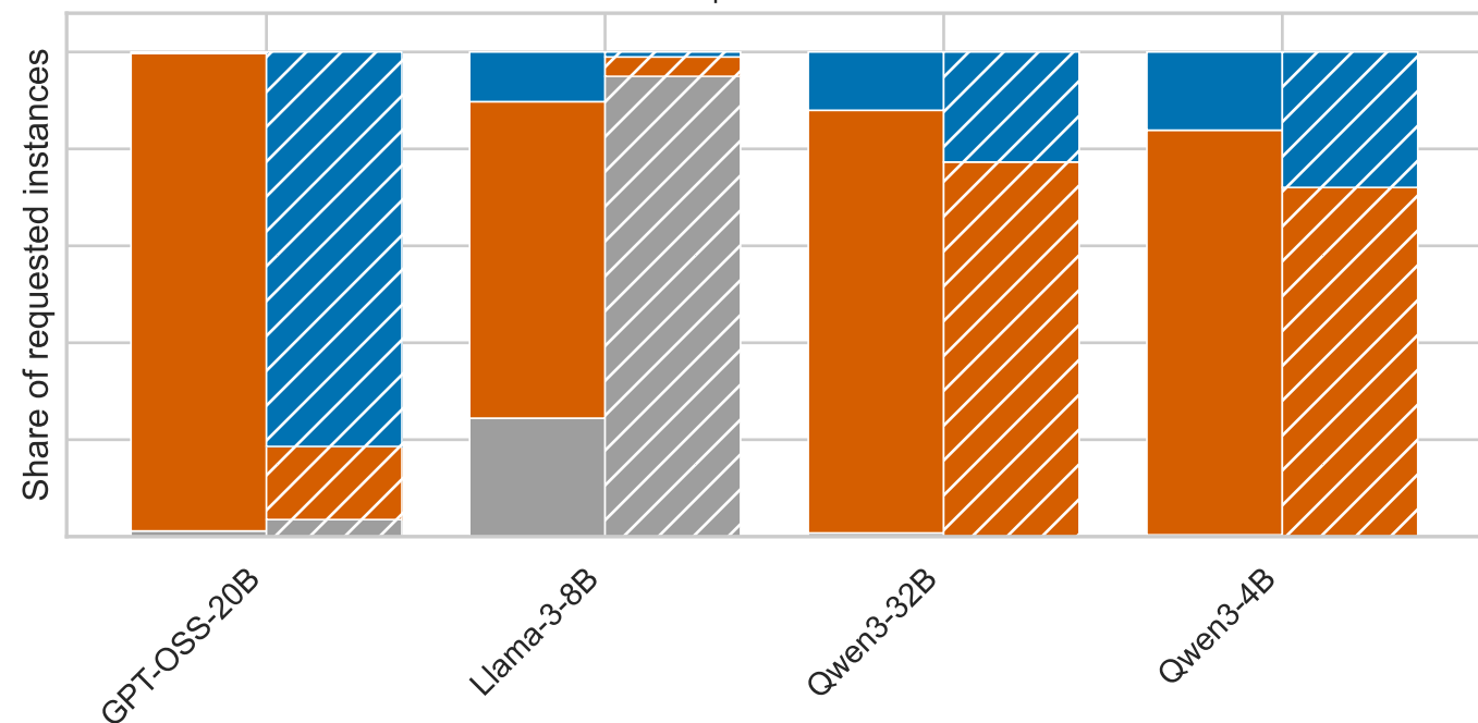
Setwise | TREC-DL-2020
