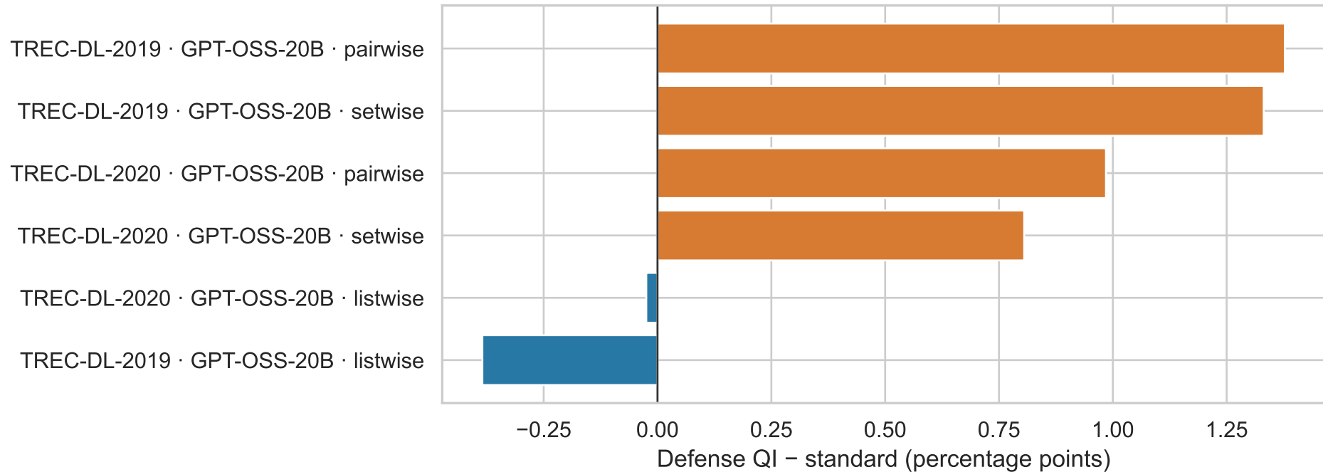
Query-injection defense effect on close-attack success
