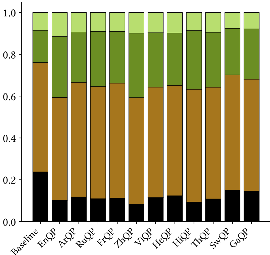
Relevance Score
