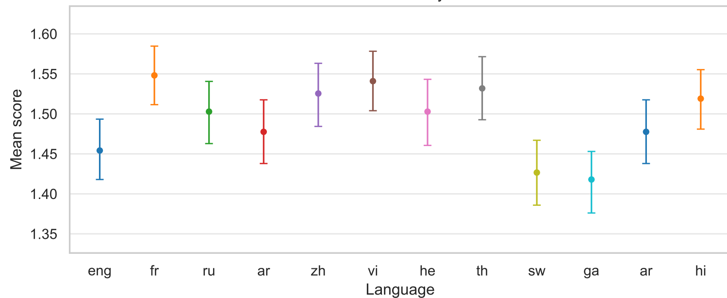
Contextuality
