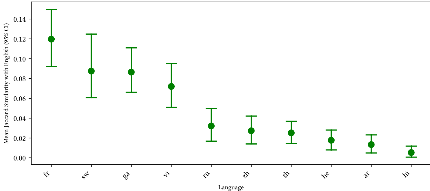
Mean Jaccard Similarity of Query BOW Sets between English and Other Languages (95% CI)
